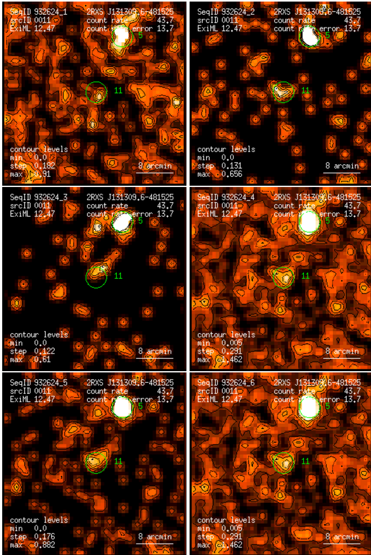
Figure 11: RASS 932624: detection 0011: band rate images, Gaussian filter: (1) PSPC channels 11 – 41, (2) 52 – 90, (3) 91 – 201, (4) 11 – 235, (5) 52 – 201, (6) 11 – 201. Broad band rates in counts/ks. Band rate contour levels in counts/ks/arcmin 2 .
