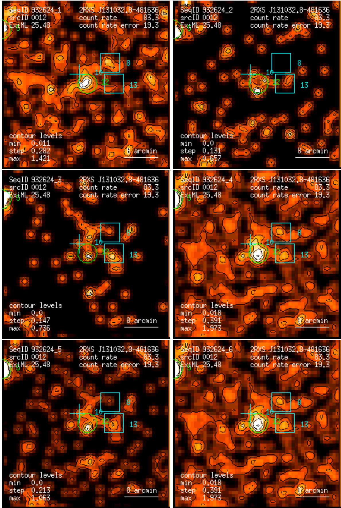
Figure 12: RASS 932624: detection 0012: band rate images, Gaussian filter: (1) PSPC channels 11 – 41, (2) 52 – 90, (3) 91 – 201, (4) 11 – 235, (5) 52 – 201, (6) 11 – 201. Broad band rates in counts/ks. Band rate contour levels in counts/ks/arcmin 2 .
