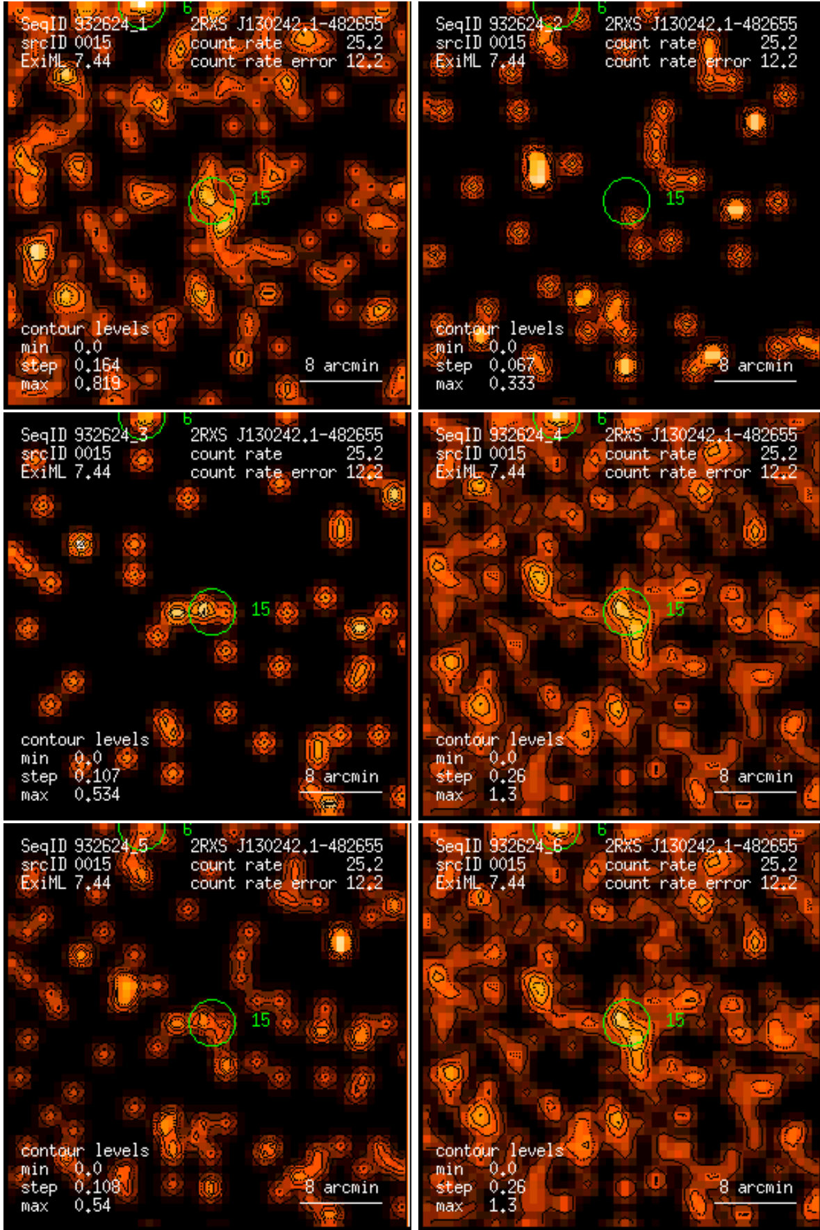
Figure 15: RASS 932624: detection 0015: band rate images, Gaussian filter: (1) PSPC channels 11 – 41, (2) 52 – 90, (3) 91 – 201, (4) 11 – 235, (5) 52 – 201, (6) 11 – 201. Broad band rates in counts/ks. Band rate contour levels in counts/ks/arcmin 2 .
