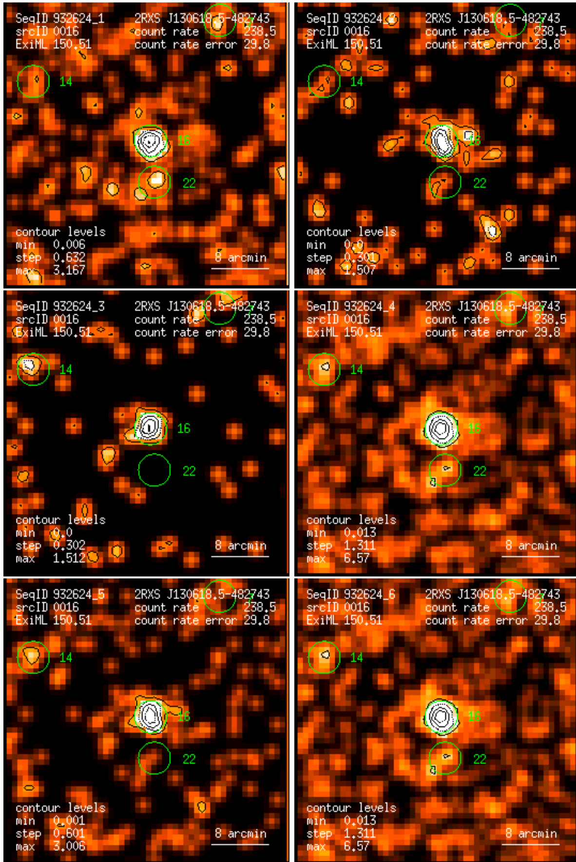
Figure 16: RASS 932624: detection 0016: band rate images, Gaussian filter: (1) PSPC channels 11 – 41, (2) 52 – 90, (3) 91 – 201, (4) 11 – 235, (5) 52 – 201, (6) 11 – 201. Broad band rates in counts/ks. Band rate contour levels in counts/ks/arcmin 2 .
