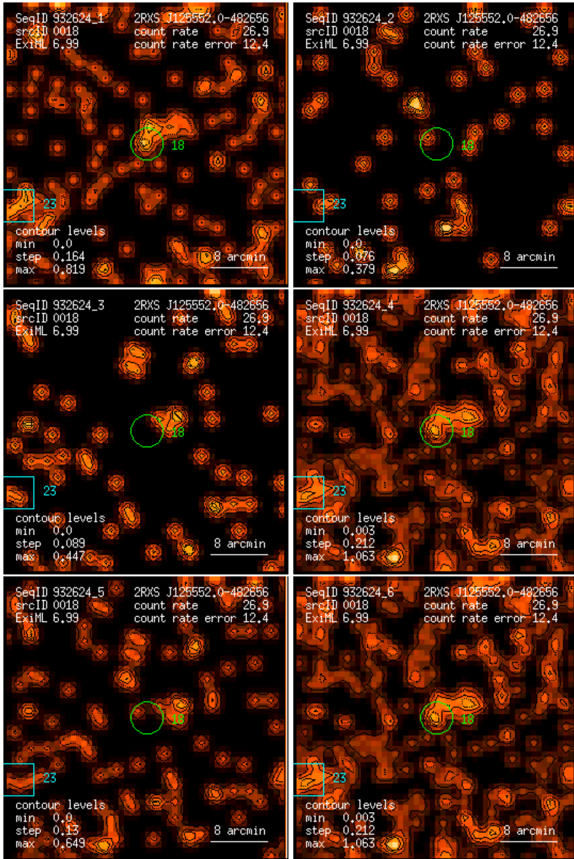
Figure 18: RASS 932624: detection 0018: band rate images, Gaussian filter: (1) PSPC channels 11 – 41, (2) 52 – 90, (3) 91 – 201, (4) 11 – 235, (5) 52 – 201, (6) 11 – 201. Broad band rates in counts/ks. Band rate contour levels in counts/ks/arcmin 2 .
