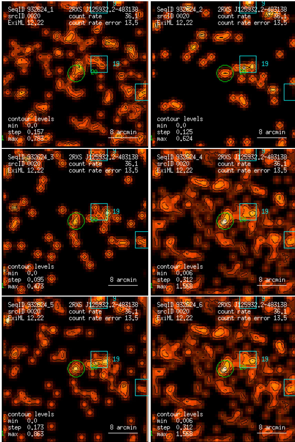
Figure 20: RASS 932624: detection 0020: band rate images, Gaussian filter: (1) PSPC channels 11 – 41, (2) 52 – 90, (3) 91 – 201, (4) 11 – 235, (5) 52 – 201, (6) 11 – 201. Broad band rates in counts/ks. Band rate contour levels in counts/ks/arcmin 2 .
