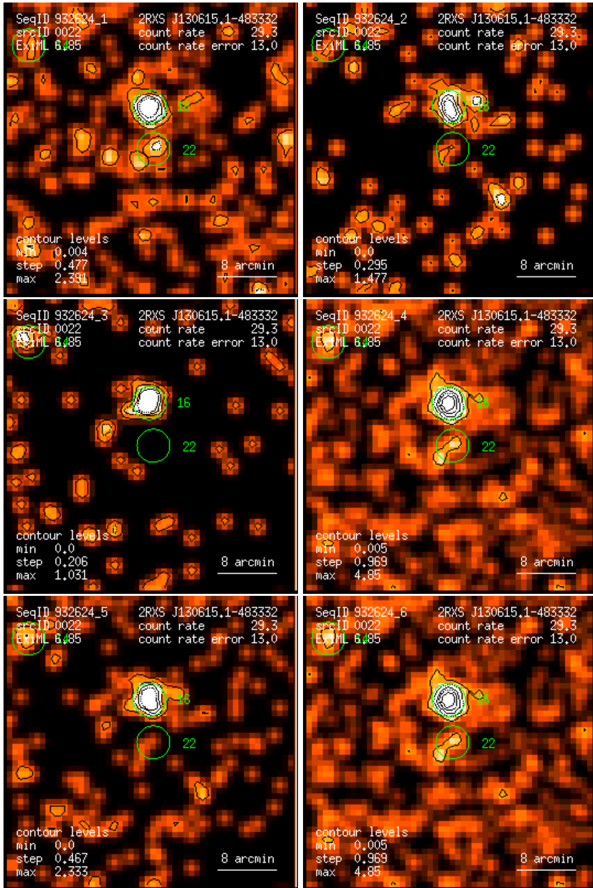
Figure 22: RASS 932624: detection 0022: band rate images, Gaussian filter: (1) PSPC channels 11 – 41, (2) 52 – 90, (3) 91 – 201, (4) 11 – 235, (5) 52 – 201, (6) 11 – 201. Broad band rates in counts/ks. Band rate contour levels in counts/ks/arcmin 2 .
