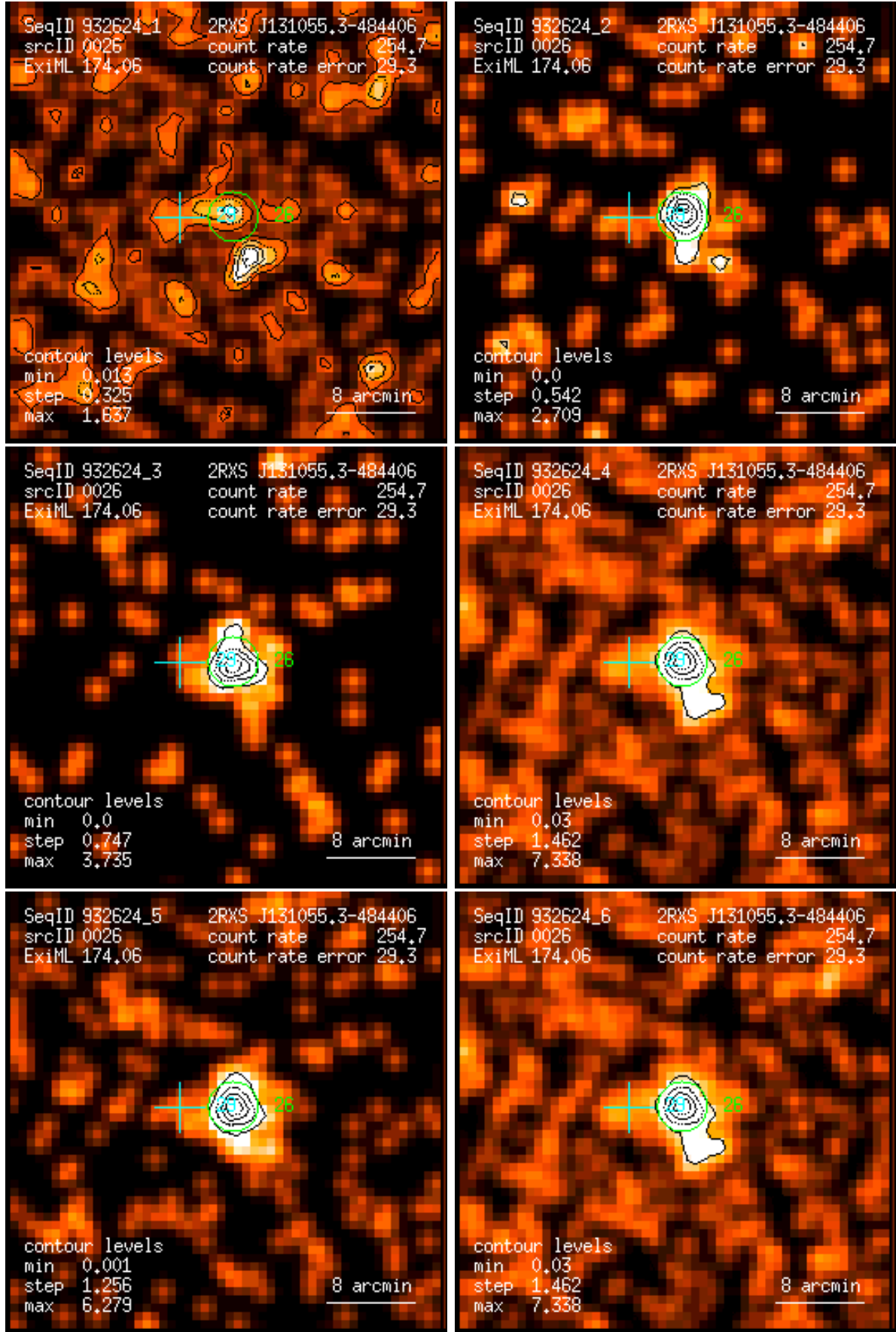
Figure 26: RASS 932624: detection 0026: band rate images, Gaussian filter: (1) PSPC channels 11 – 41, (2) 52 – 90, (3) 91 – 201, (4) 11 – 235, (5) 52 – 201, (6) 11 – 201. Broad band rates in counts/ks. Band rate contour levels in counts/ks/arcmin 2 .
