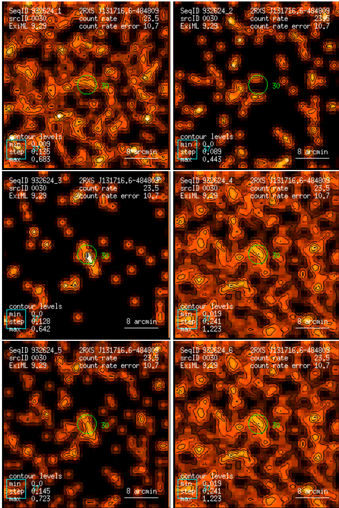
Figure 30: RASS 932624: detection 0030: band rate images, Gaussian filter: (1) PSPC channels 11 – 41, (2) 52 – 90, (3) 91 – 201, (4) 11 – 235, (5) 52 – 201, (6) 11 – 201. Broad band rates in counts/ks. Band rate contour levels in counts/ks/arcmin 2 .
