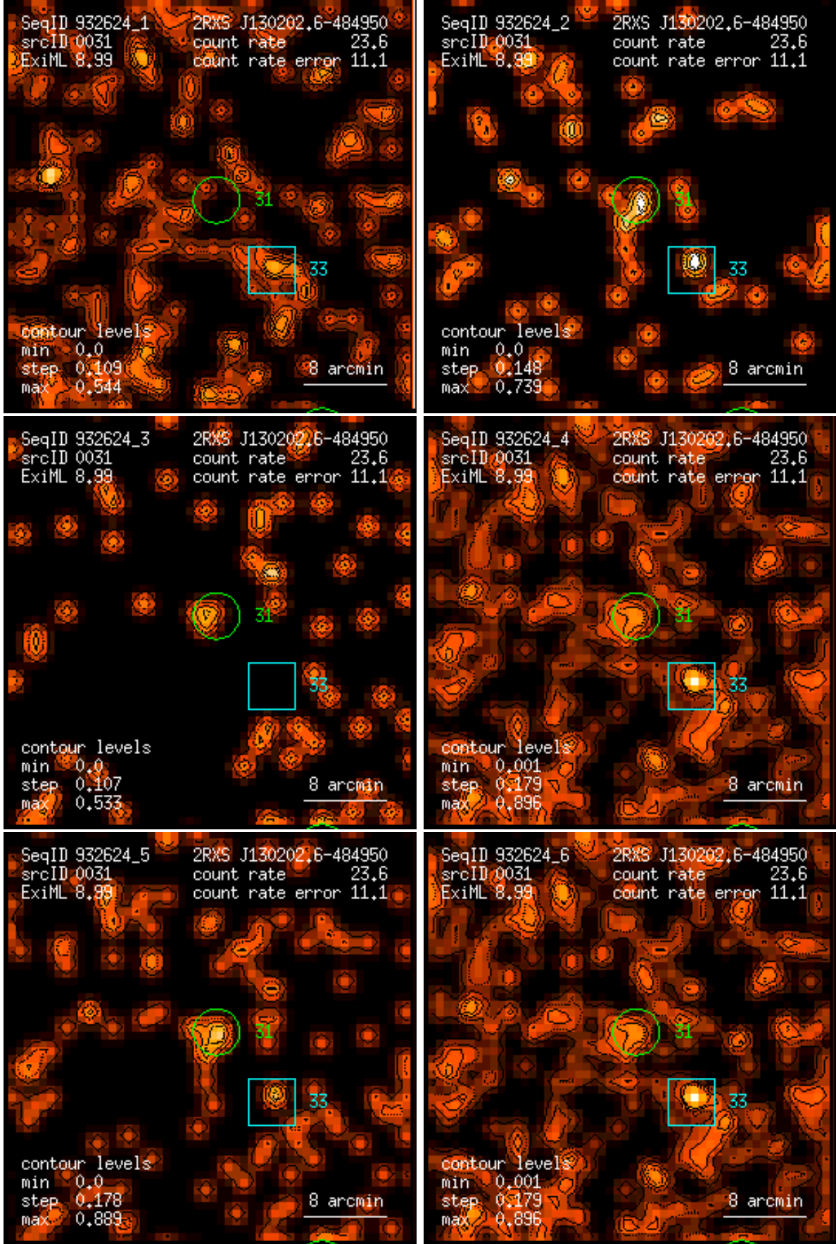
Figure 31: RASS 932624: detection 0031: band rate images, Gaussian filter: (1) PSPC channels 11 – 41, (2) 52 – 90, (3) 91 – 201, (4) 11 – 235, (5) 52 – 201, (6) 11 – 201. Broad band rates in counts/ks. Band rate contour levels in counts/ks/arcmin 2 .
