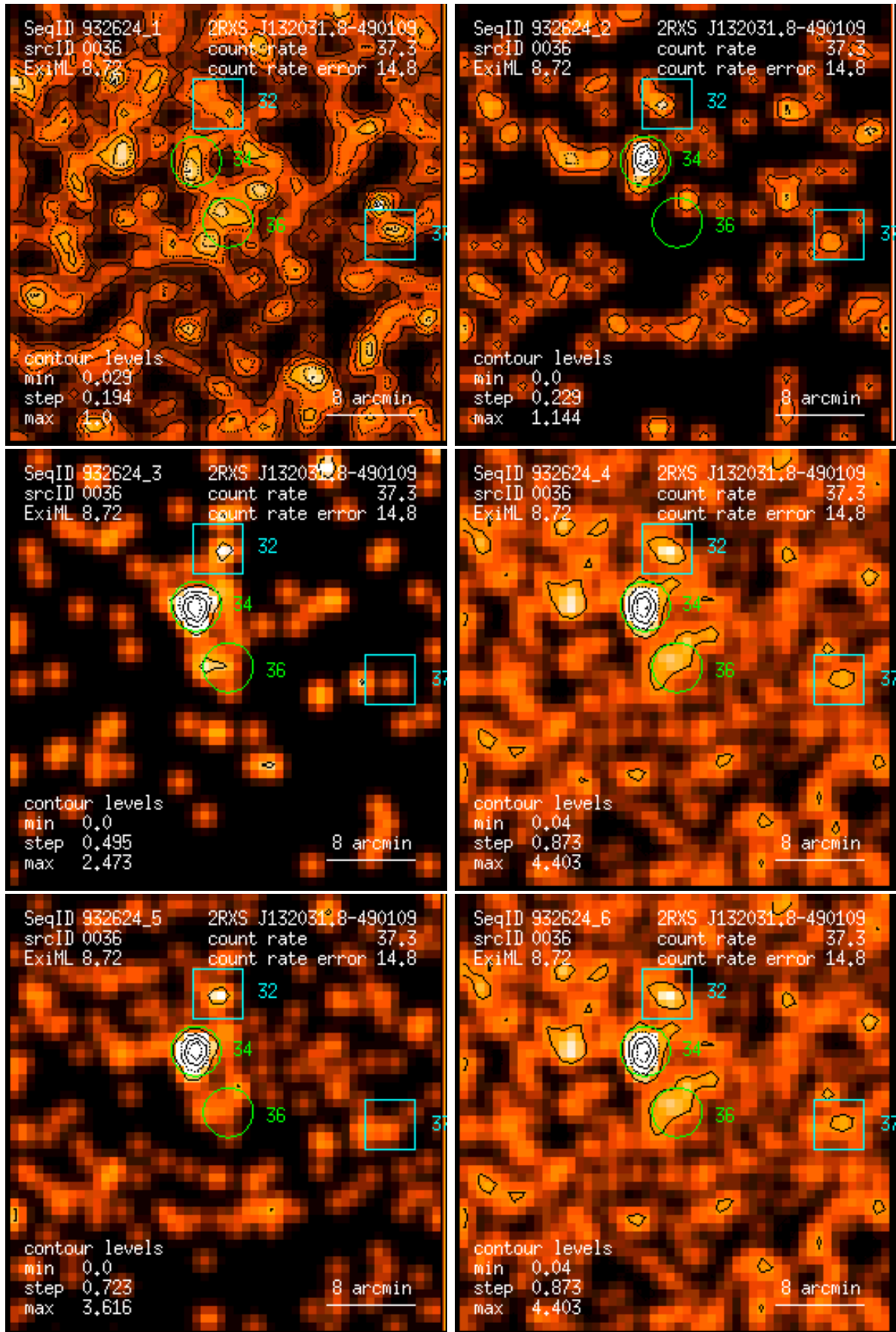
Figure 36: RASS 932624: detection 0036: band rate images, Gaussian filter: (1) PSPC channels 11 – 41, (2) 52 – 90, (3) 91 – 201, (4) 11 – 235, (5) 52 – 201, (6) 11 – 201. Broad band rates in counts/ks. Band rate contour levels in counts/ks/arcmin 2 .
