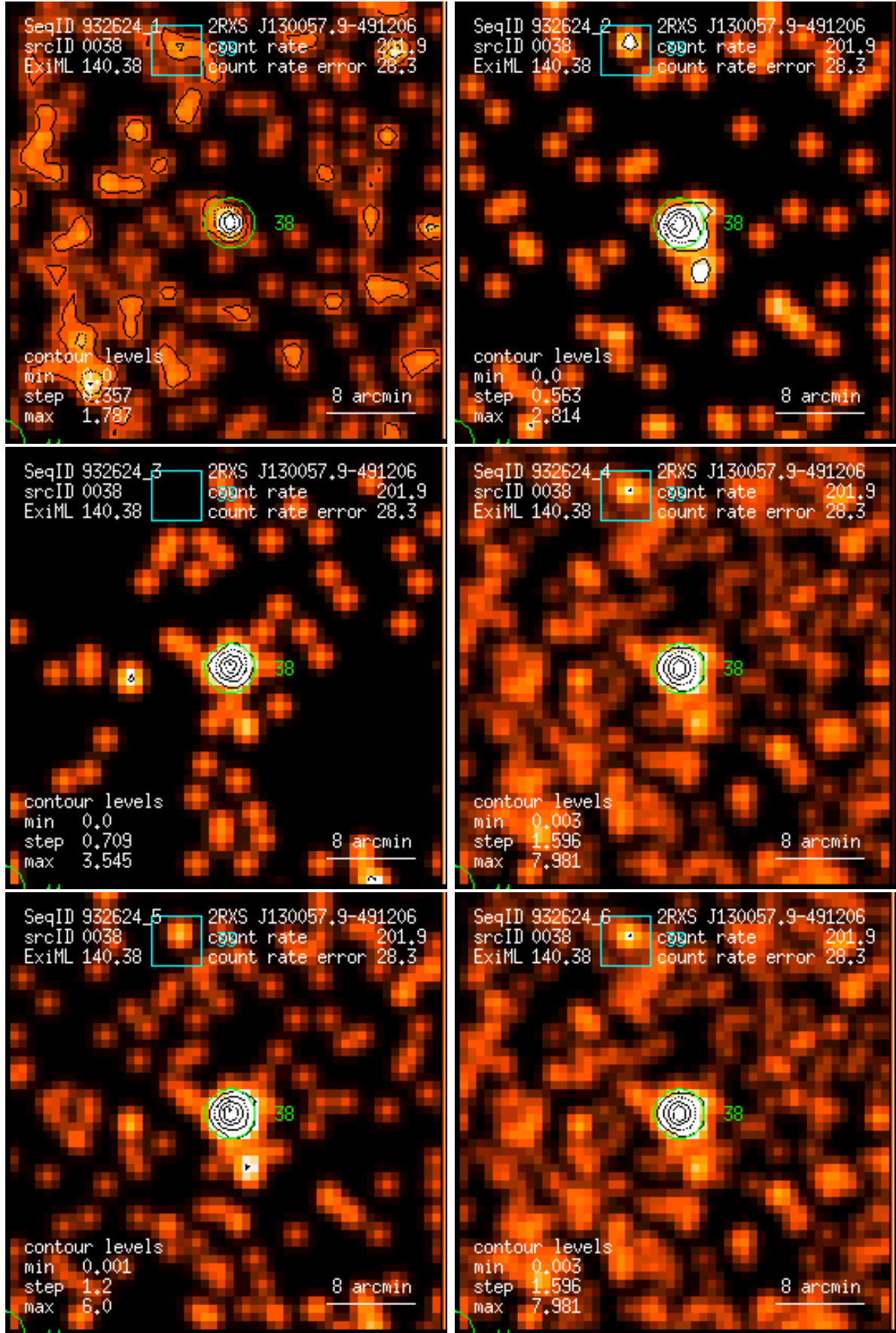
Figure 38: RASS 932624: detection 0038: band rate images, Gaussian filter: (1) PSPC channels 11 – 41, (2) 52 – 90, (3) 91 – 201, (4) 11 – 235, (5) 52 – 201, (6) 11 – 201. Broad band rates in counts/ks. Band rate contour levels in counts/ks/arcmin 2 .
