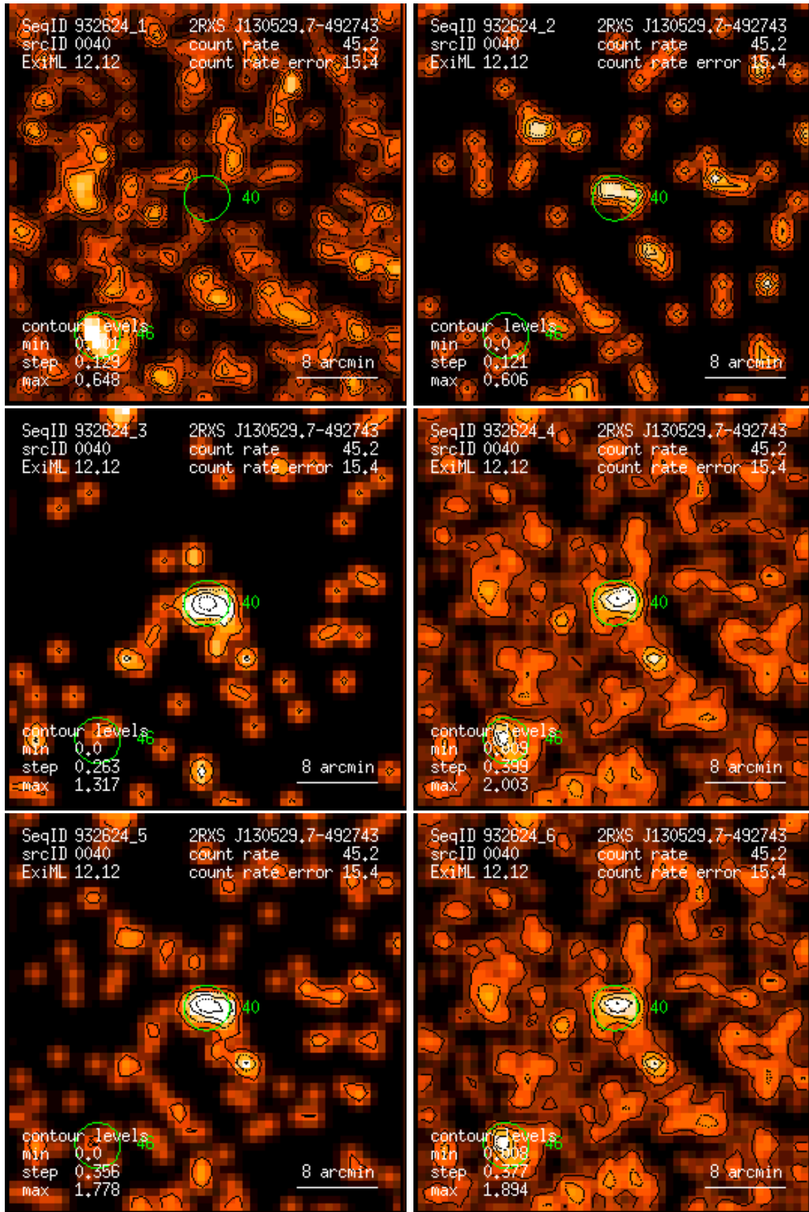
Figure 40: RASS 932624: detection 0040: band rate images, Gaussian filter: (1) PSPC channels 11 – 41, (2) 52 – 90, (3) 91 – 201, (4) 11 – 235, (5) 52 – 201, (6) 11 – 201. Broad band rates in counts/ks. Band rate contour levels in counts/ks/arcmin 2 .
