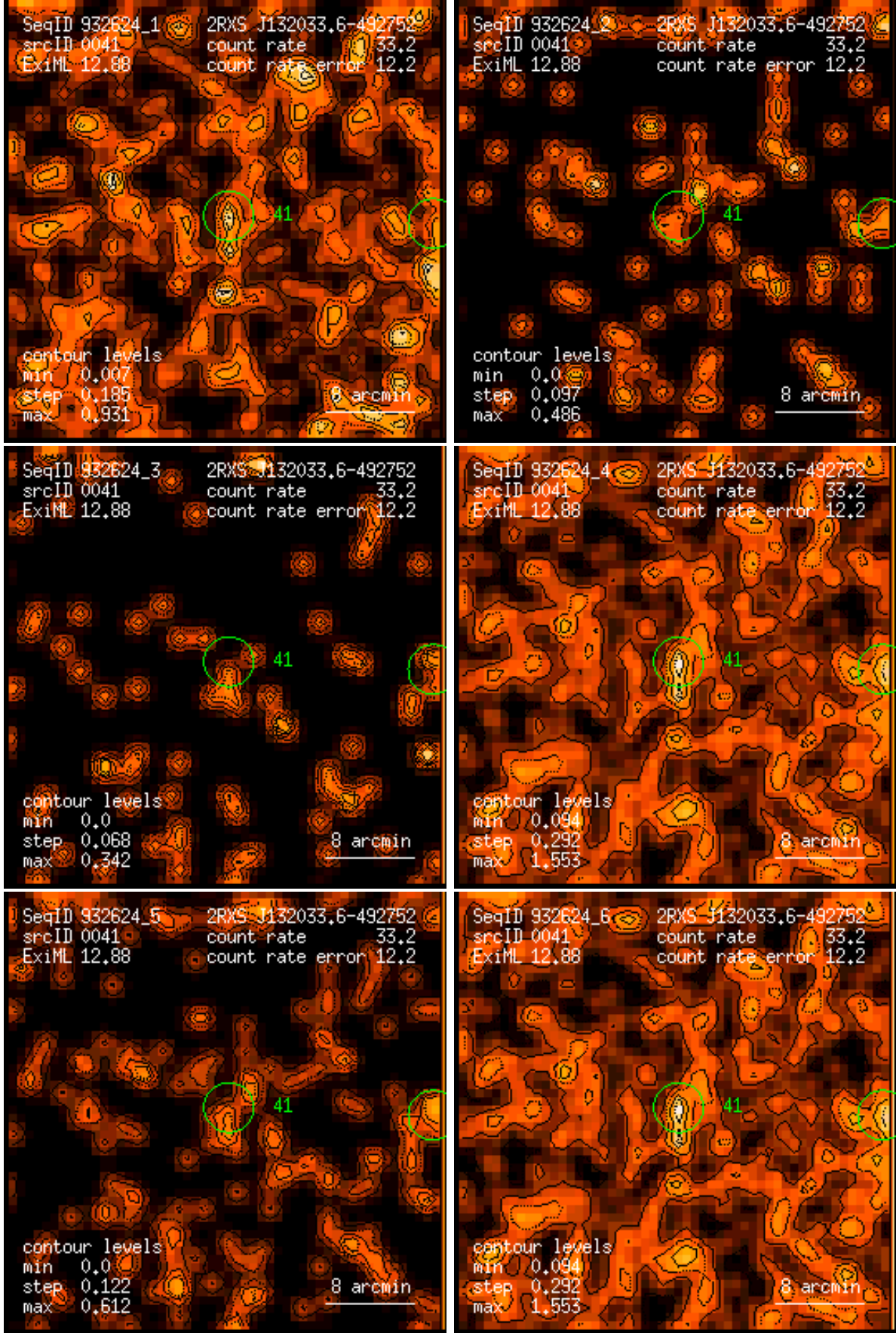
Figure 41: RASS 932624: detection 0041: band rate images, Gaussian filter: (1) PSPC channels 11 – 41, (2) 52 – 90, (3) 91 – 201, (4) 11 – 235, (5) 52 – 201, (6) 11 – 201. Broad band rates in counts/ks. Band rate contour levels in counts/ks/arcmin 2 .
