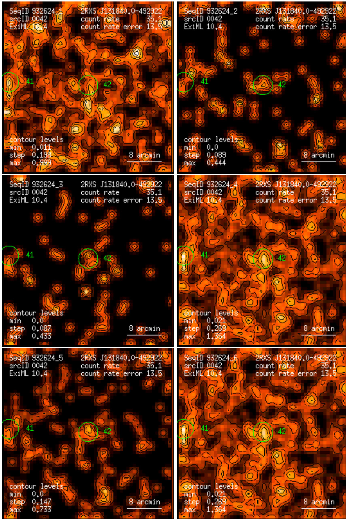
Figure 42: RASS 932624: detection 0042: band rate images, Gaussian filter: (1) PSPC channels 11 – 41, (2) 52 – 90, (3) 91 – 201, (4) 11 – 235, (5) 52 – 201, (6) 11 – 201. Broad band rates in counts/ks. Band rate contour levels in counts/ks/arcmin 2 .
