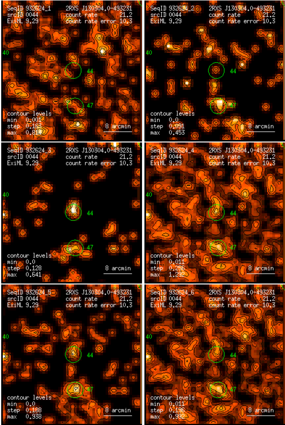
Figure 44: RASS 932624: detection 0044: band rate images, Gaussian filter: (1) PSPC channels 11 – 41, (2) 52 – 90, (3) 91 – 201, (4) 11 – 235, (5) 52 – 201, (6) 11 – 201. Broad band rates in counts/ks. Band rate contour levels in counts/ks/arcmin 2 .
