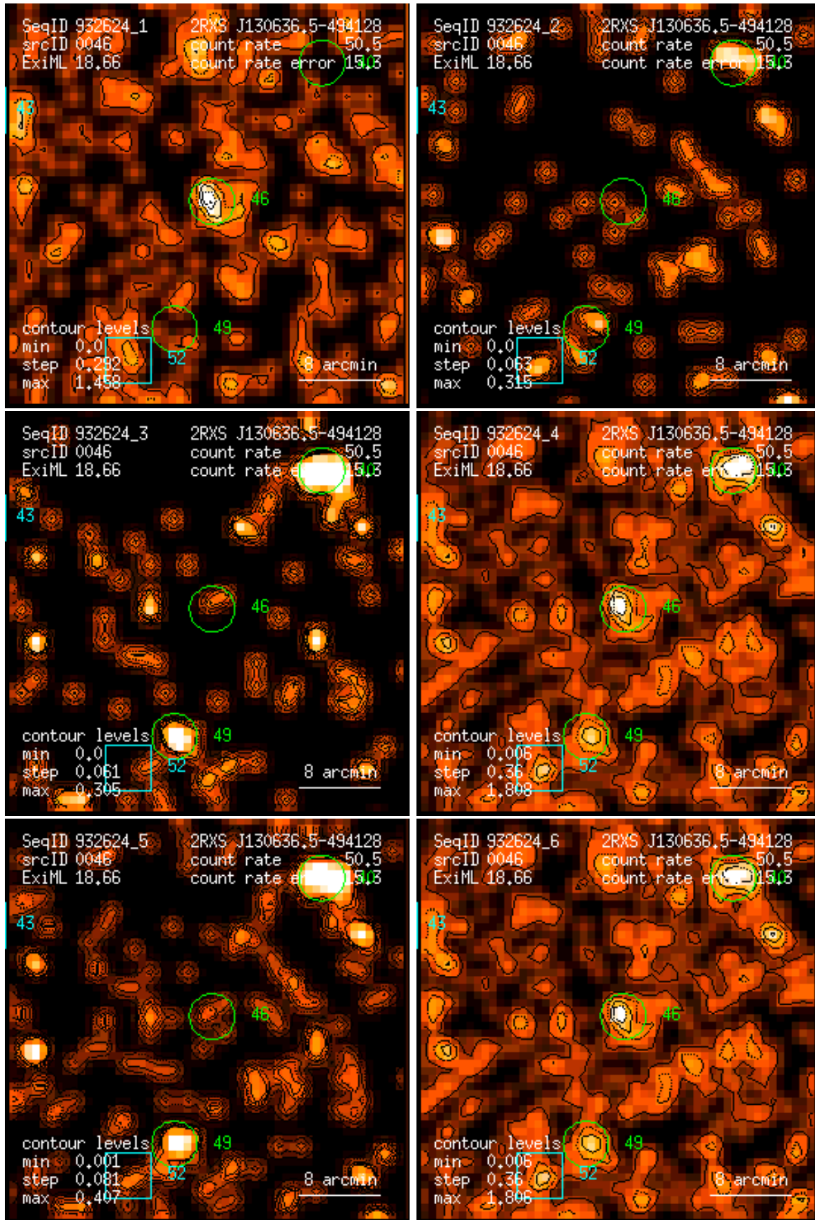
Figure 46: RASS 932624: detection 0046: band rate images, Gaussian filter: (1) PSPC channels 11 – 41, (2) 52 – 90, (3) 91 – 201, (4) 11 – 235, (5) 52 – 201, (6) 11 – 201. Broad band rates in counts/ks. Band rate contour levels in counts/ks/arcmin 2 .
