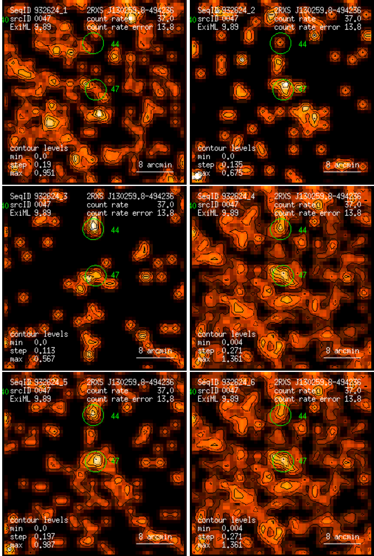
Figure 47: RASS 932624: detection 0047: band rate images, Gaussian filter: (1) PSPC channels 11 – 41, (2) 52 – 90, (3) 91 – 201, (4) 11 – 235, (5) 52 – 201, (6) 11 – 201. Broad band rates in counts/ks. Band rate contour levels in counts/ks/arcmin 2 .
