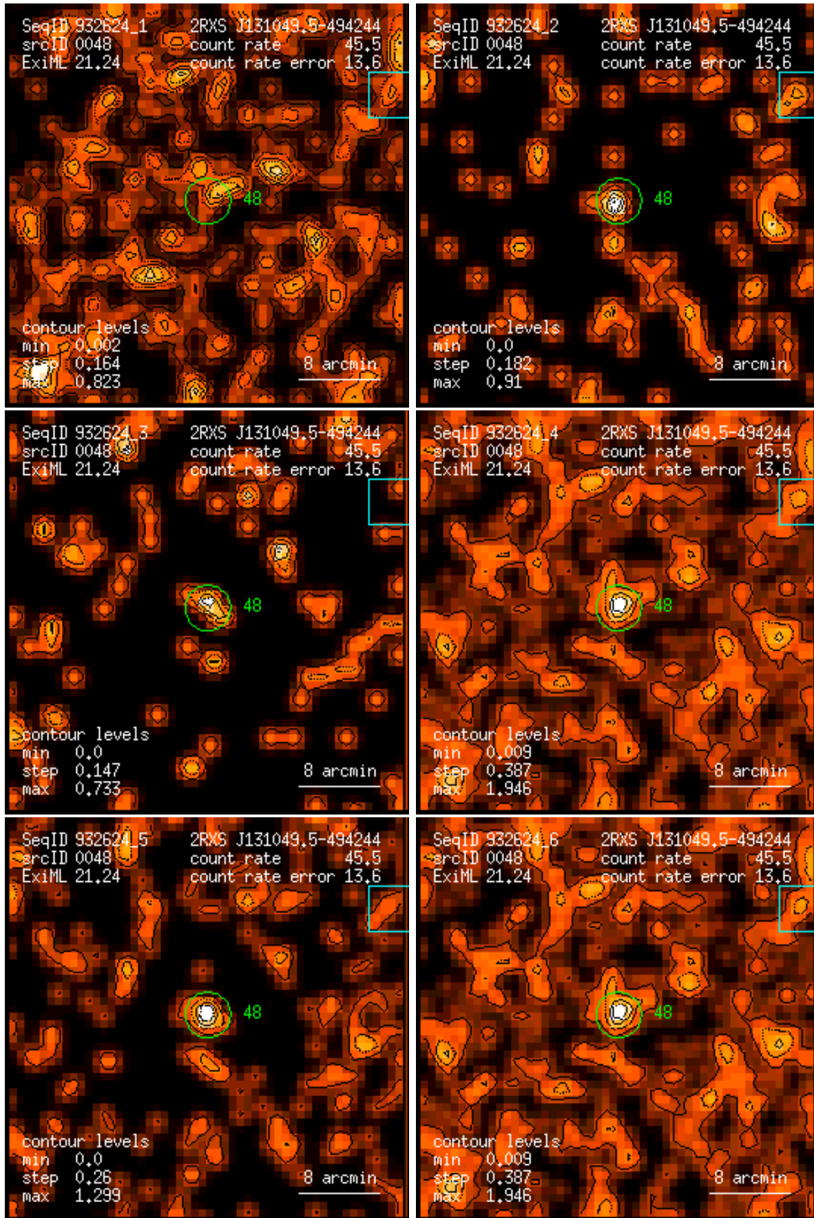
Figure 48: RASS 932624: detection 0048: band rate images, Gaussian filter: (1) PSPC channels 11 – 41, (2) 52 – 90, (3) 91 – 201, (4) 11 – 235, (5) 52 – 201, (6) 11 – 201. Broad band rates in counts/ks. Band rate contour levels in counts/ks/arcmin 2 .
