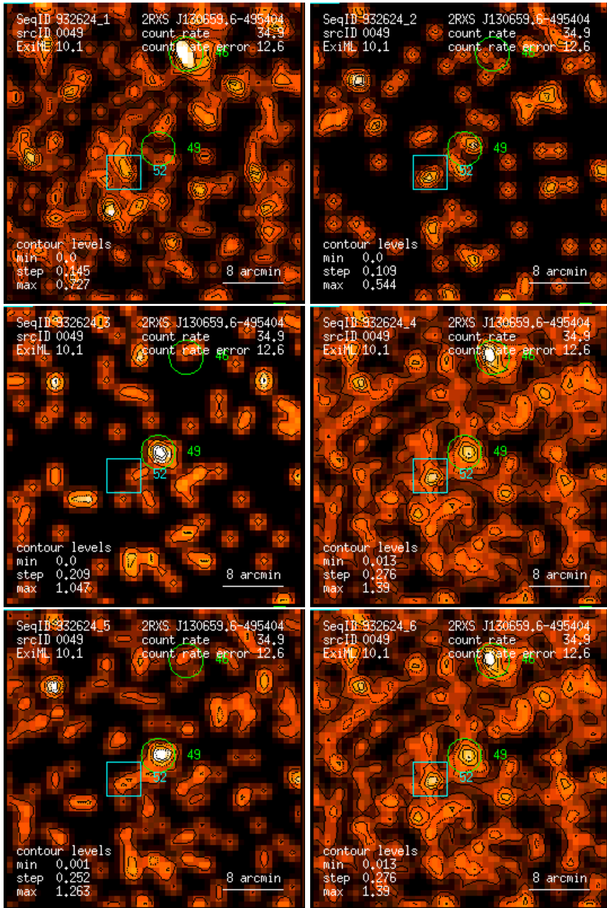
Figure 49: RASS 932624: detection 0049: band rate images, Gaussian filter: (1) PSPC channels 11 – 41, (2) 52 – 90, (3) 91 – 201, (4) 11 – 235, (5) 52 – 201, (6) 11 – 201. Broad band rates in counts/ks. Band rate contour levels in counts/ks/arcmin 2 .
