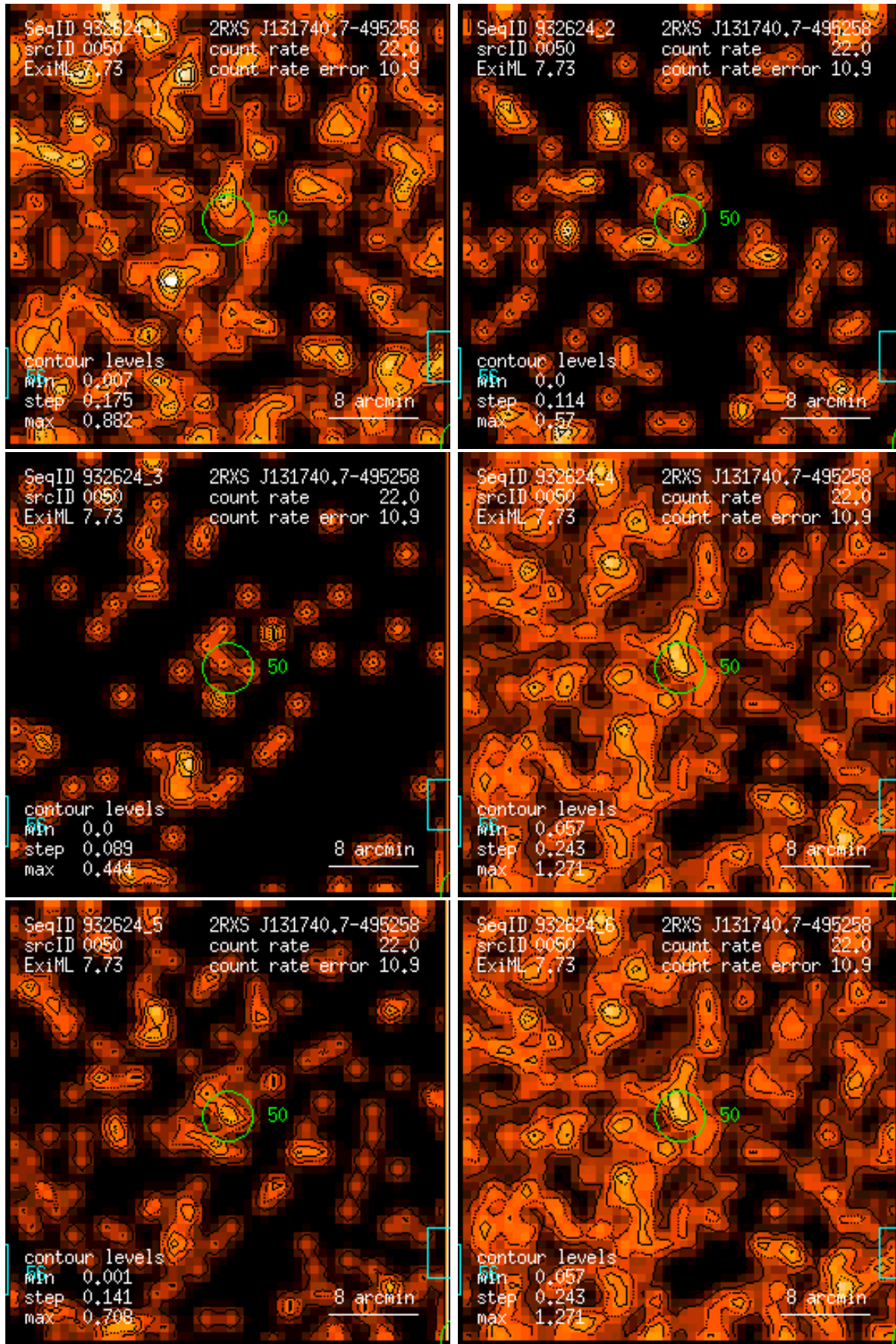
Figure 50: RASS 932624: detection 0050: band rate images, Gaussian filter: (1) PSPC channels 11 – 41, (2) 52 – 90, (3) 91 – 201, (4) 11 – 235, (5) 52 – 201, (6) 11 – 201. Broad band rates in counts/ks. Band rate contour levels in counts/ks/arcmin 2 .
