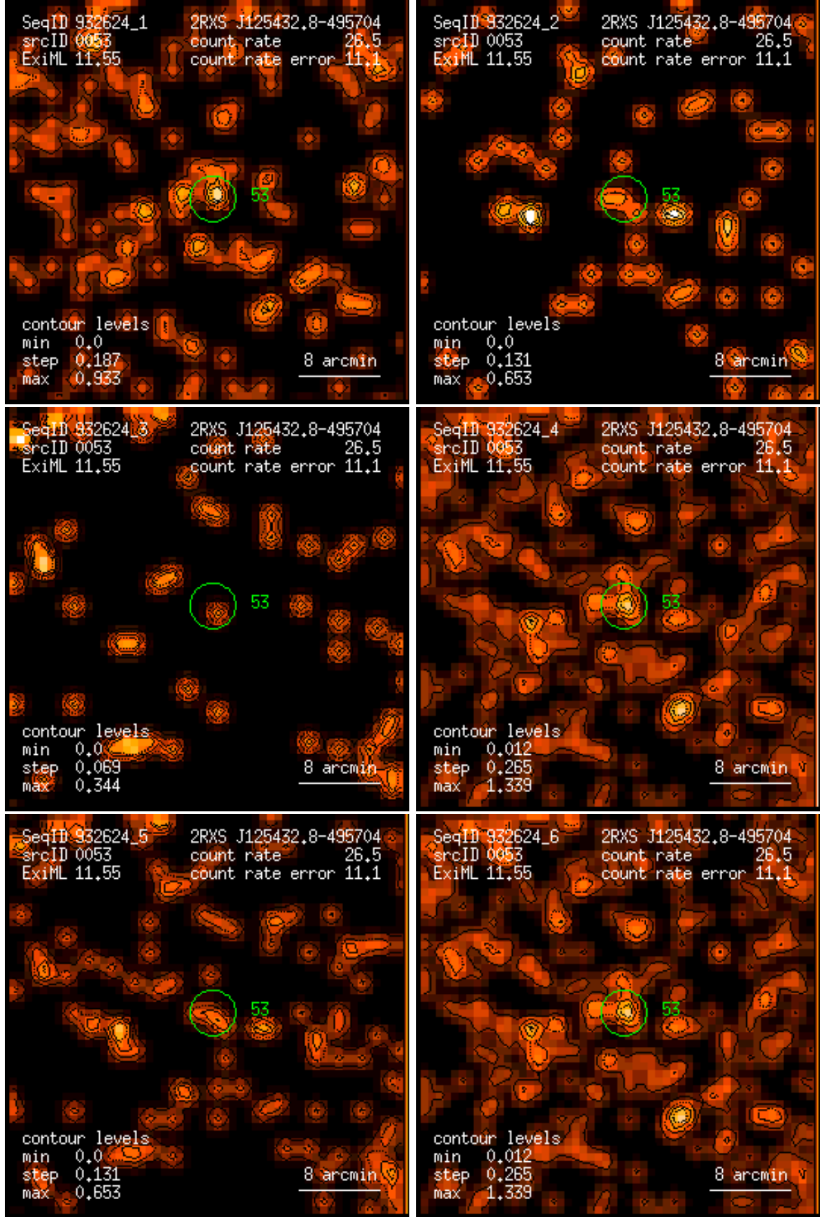
Figure 53: RASS 932624: detection 0053: band rate images, Gaussian filter: (1) PSPC channels 11 – 41, (2) 52 – 90, (3) 91 – 201, (4) 11 – 235, (5) 52 – 201, (6) 11 – 201. Broad band rates in counts/ks. Band rate contour levels in counts/ks/arcmin 2 .
