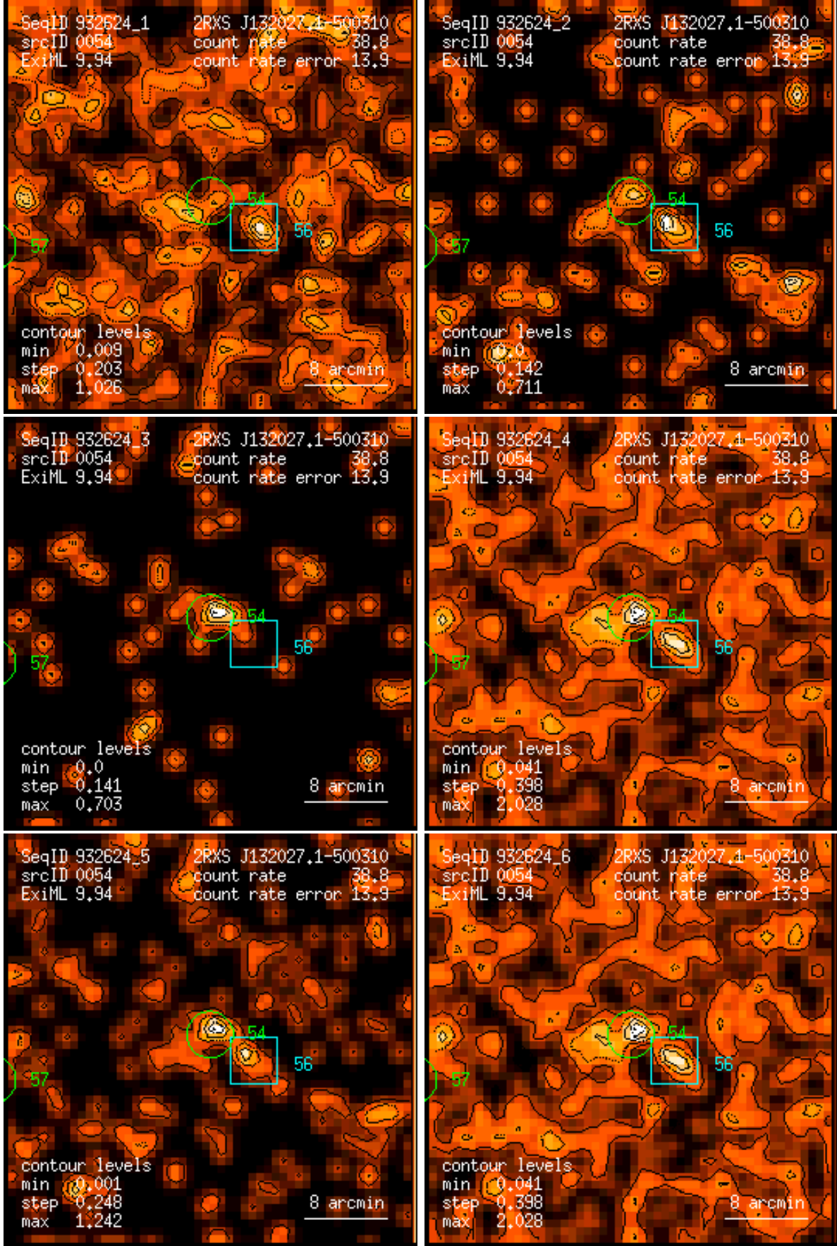
Figure 54: RASS 932624: detection 0054: band rate images, Gaussian filter: (1) PSPC channels 11 – 41, (2) 52 – 90, (3) 91 – 201, (4) 11 – 235, (5) 52 – 201, (6) 11 – 201. Broad band rates in counts/ks. Band rate contour levels in counts/ks/arcmin 2 .
