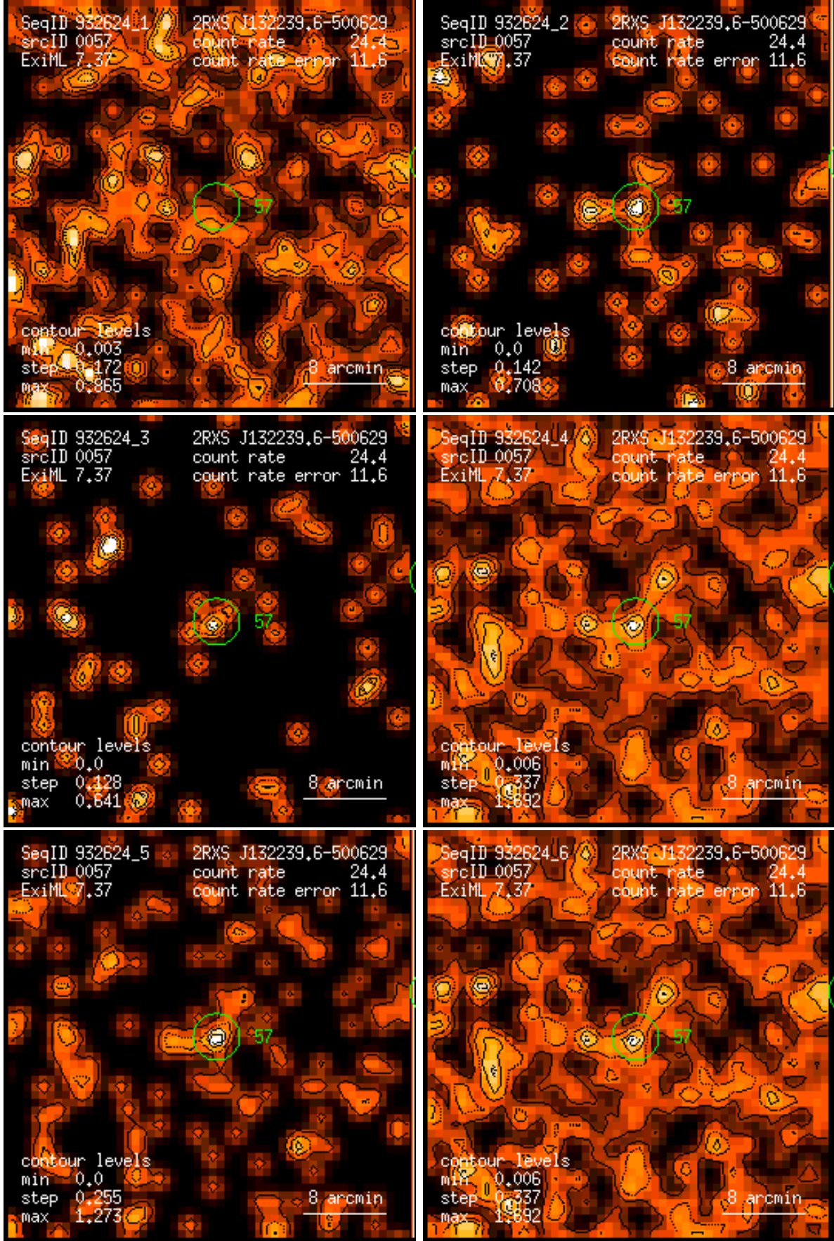
Figure 57: RASS 932624: detection 0057: band rate images, Gaussian filter: (1) PSPC channels 11 – 41, (2) 52 – 90, (3) 91 – 201, (4) 11 – 235, (5) 52 – 201, (6) 11 – 201. Broad band rates in counts/ks. Band rate contour levels in counts/ks/arcmin 2 .
