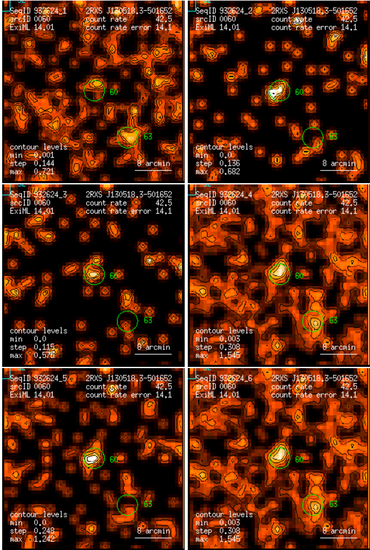
Figure 60: RASS 932624: detection 0060: band rate images, Gaussian filter: (1) PSPC channels 11 – 41, (2) 52 – 90, (3) 91 – 201, (4) 11 – 235, (5) 52 – 201, (6) 11 – 201. Broad band rates in counts/ks. Band rate contour levels in counts/ks/arcmin 2 .
