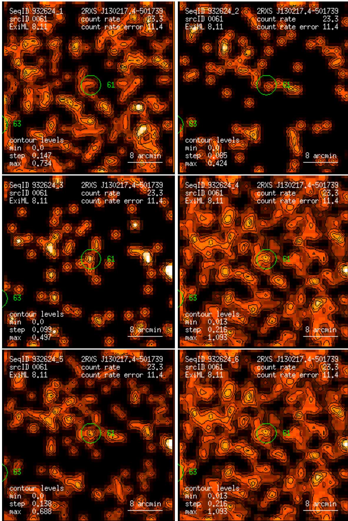
Figure 61: RASS 932624: detection 0061: band rate images, Gaussian filter: (1) PSPC channels 11 – 41, (2) 52 – 90, (3) 91 – 201, (4) 11 – 235, (5) 52 – 201, (6) 11 – 201. Broad band rates in counts/ks. Band rate contour levels in counts/ks/arcmin 2 .
