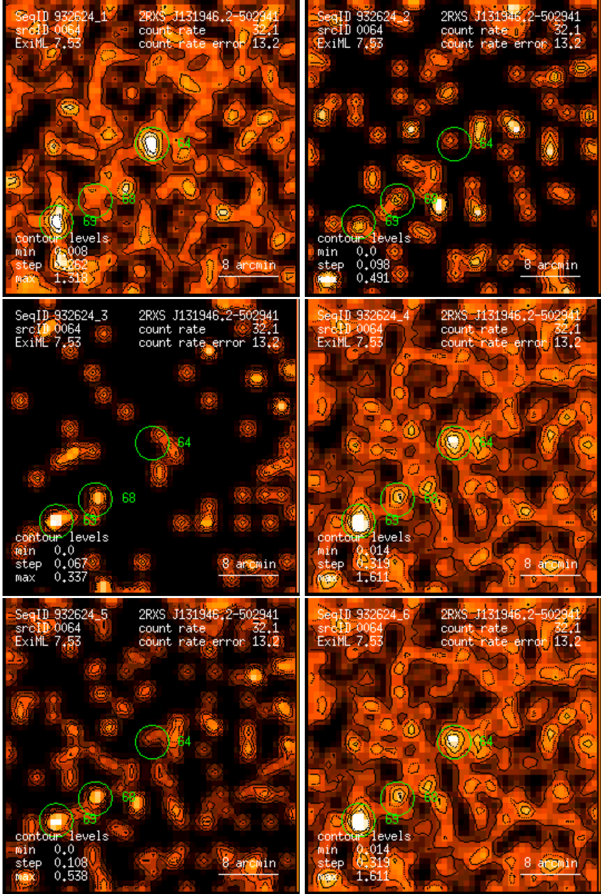
Figure 64: RASS 932624: detection 0064: band rate images, Gaussian filter: (1) PSPC channels 11 – 41, (2) 52 – 90, (3) 91 – 201, (4) 11 – 235, (5) 52 – 201, (6) 11 – 201. Broad band rates in counts/ks. Band rate contour levels in counts/ks/arcmin 2 .
