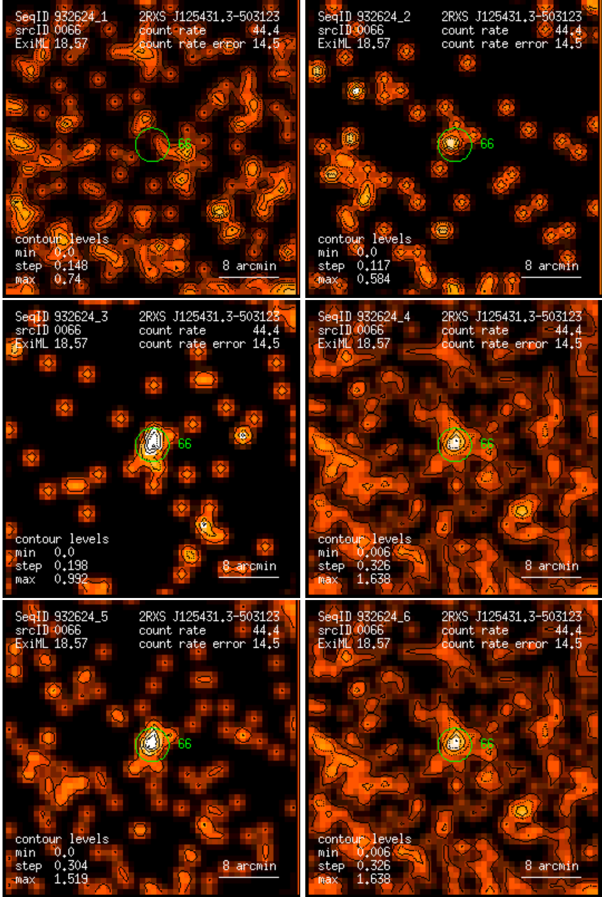
Figure 66: RASS 932624: detection 0066: band rate images, Gaussian filter: (1) PSPC channels 11 – 41, (2) 52 – 90, (3) 91 – 201, (4) 11 – 235, (5) 52 – 201, (6) 11 – 201. Broad band rates in counts/ks. Band rate contour levels in counts/ks/arcmin 2 .
