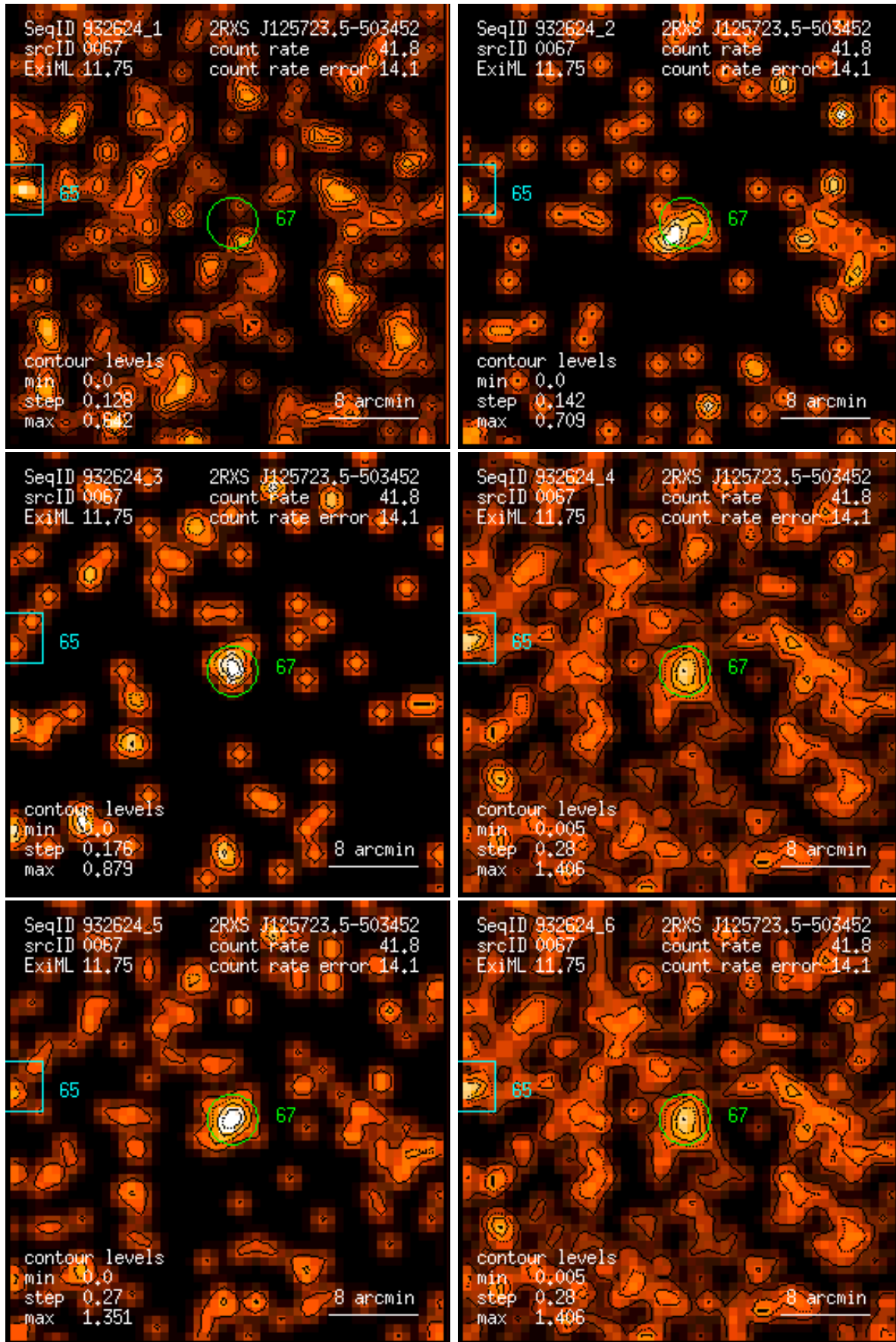
Figure 67: RASS 932624: detection 0067: band rate images, Gaussian filter: (1) PSPC channels 11 – 41, (2) 52 – 90, (3) 91 – 201, (4) 11 – 235, (5) 52 – 201, (6) 11 – 201. Broad band rates in counts/ks. Band rate contour levels in counts/ks/arcmin 2 .
