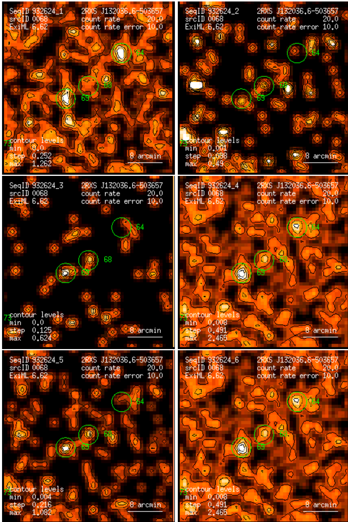
Figure 68: RASS 932624: detection 0068: band rate images, Gaussian filter: (1) PSPC channels 11 – 41, (2) 52 – 90, (3) 91 – 201, (4) 11 – 235, (5) 52 – 201, (6) 11 – 201. Broad band rates in counts/ks. Band rate contour levels in counts/ks/arcmin 2 .
