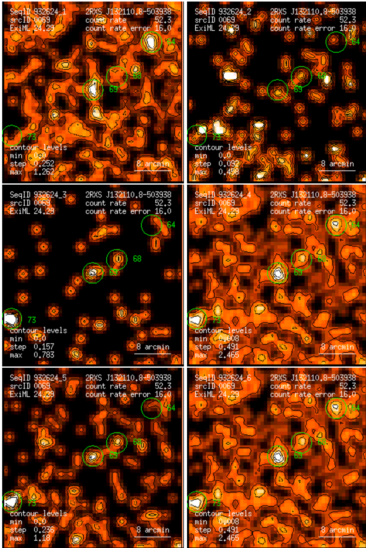
Figure 69: RASS 932624: detection 0069: band rate images, Gaussian filter: (1) PSPC channels 11 – 41, (2) 52 – 90, (3) 91 – 201, (4) 11 – 235, (5) 52 – 201, (6) 11 – 201. Broad band rates in counts/ks. Band rate contour levels in counts/ks/arcmin 2 .
