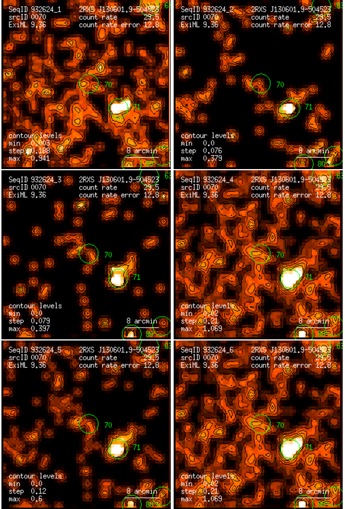
Figure 70: RASS 932624: detection 0070: band rate images, Gaussian filter: (1) PSPC channels 11 – 41, (2) 52 – 90, (3) 91 – 201, (4) 11 – 235, (5) 52 – 201, (6) 11 – 201. Broad band rates in counts/ks. Band rate contour levels in counts/ks/arcmin 2 .
