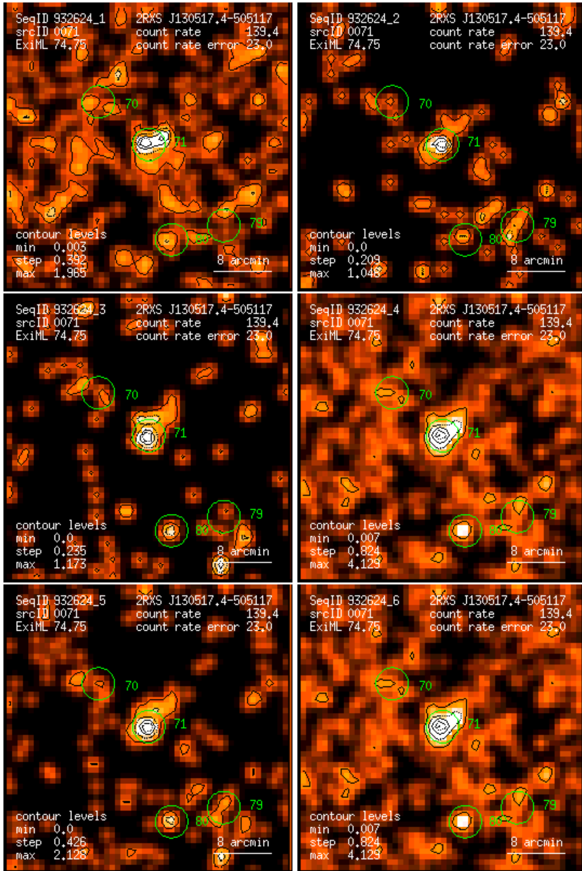
Figure 71: RASS 932624: detection 0071: band rate images, Gaussian filter: (1) PSPC channels 11 – 41, (2) 52 – 90, (3) 91 – 201, (4) 11 – 235, (5) 52 – 201, (6) 11 – 201. Broad band rates in counts/ks. Band rate contour levels in counts/ks/arcmin 2 .
