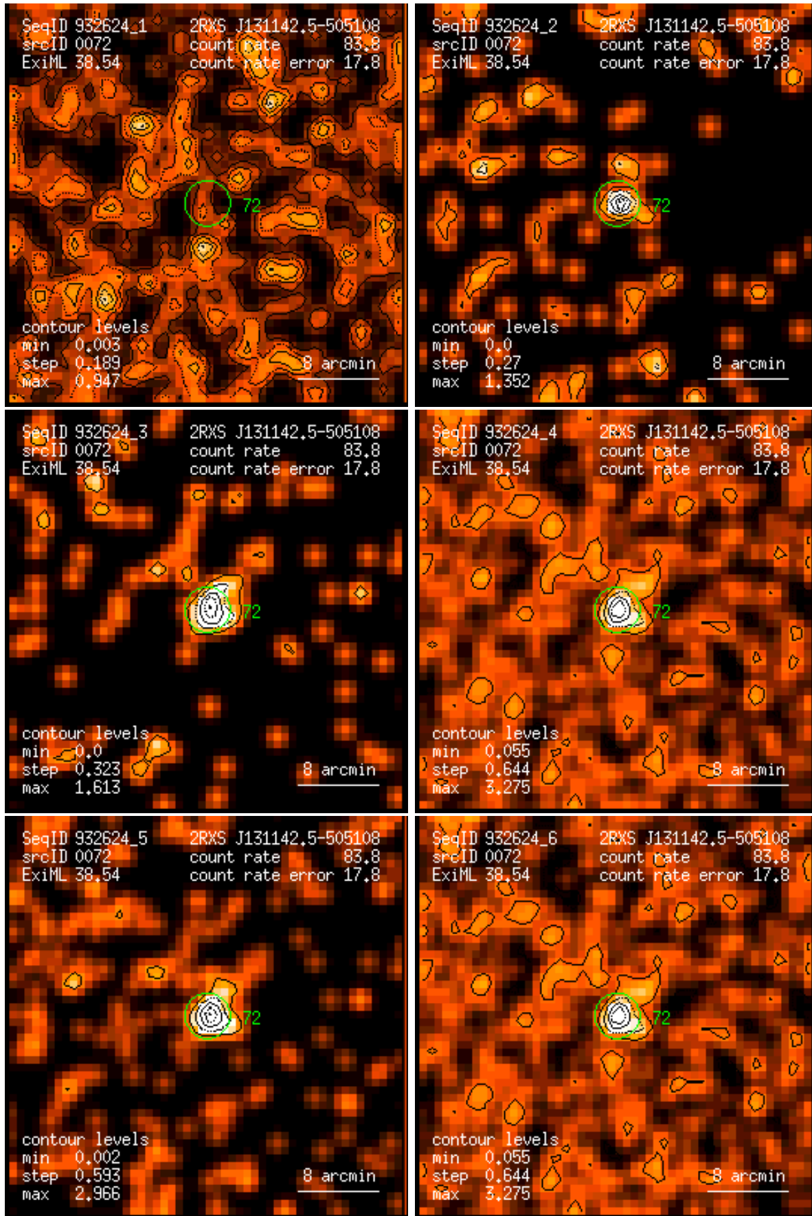
Figure 72: RASS 932624: detection 0072: band rate images, Gaussian filter: (1) PSPC channels 11 – 41, (2) 52 – 90, (3) 91 – 201, (4) 11 – 235, (5) 52 – 201, (6) 11 – 201. Broad band rates in counts/ks. Band rate contour levels in counts/ks/arcmin 2 .
