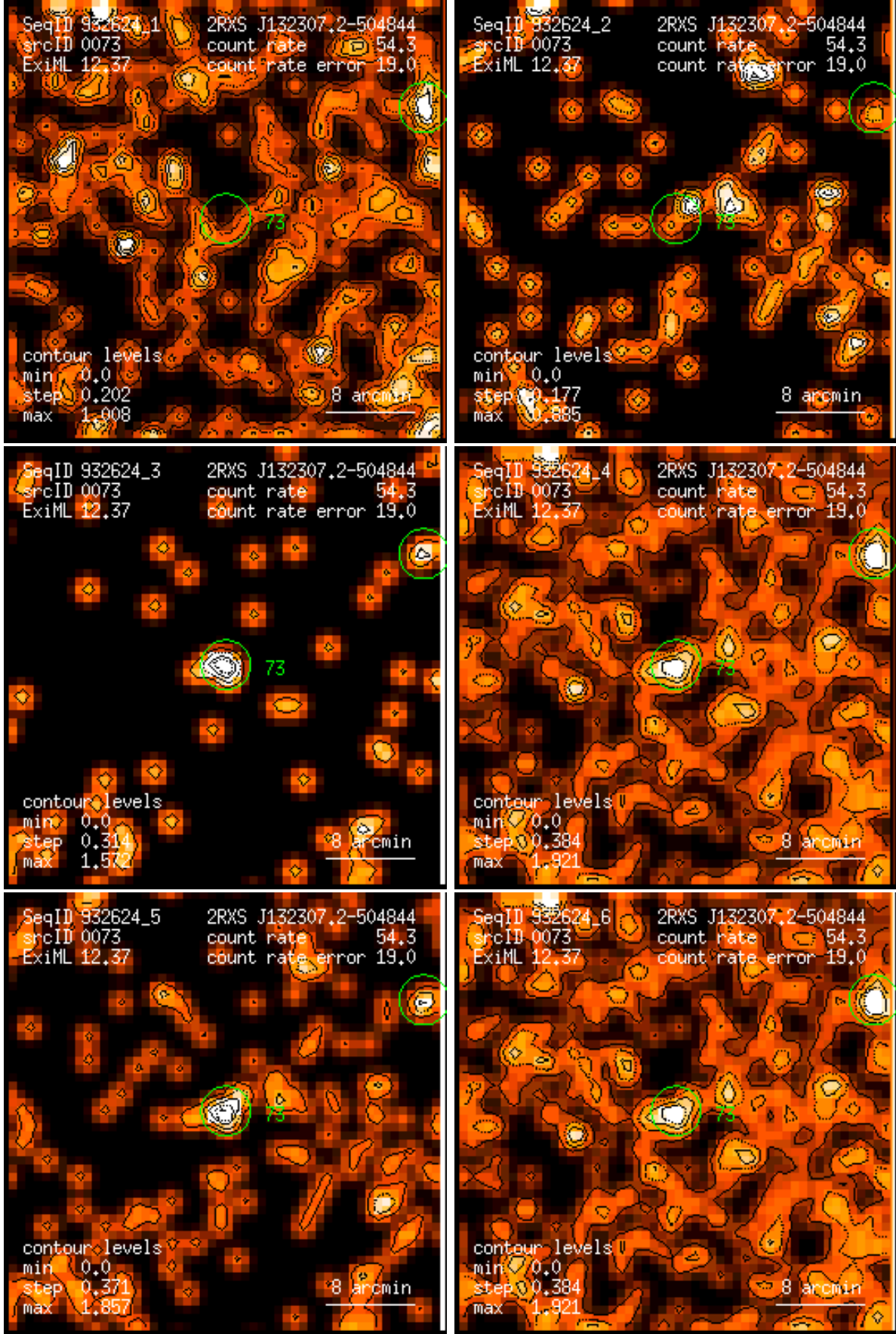
Figure 73: RASS 932624: detection 0073: band rate images, Gaussian filter: (1) PSPC channels 11 – 41, (2) 52 – 90, (3) 91 – 201, (4) 11 – 235, (5) 52 – 201, (6) 11 – 201. Broad band rates in counts/ks. Band rate contour levels in counts/ks/arcmin 2 .
