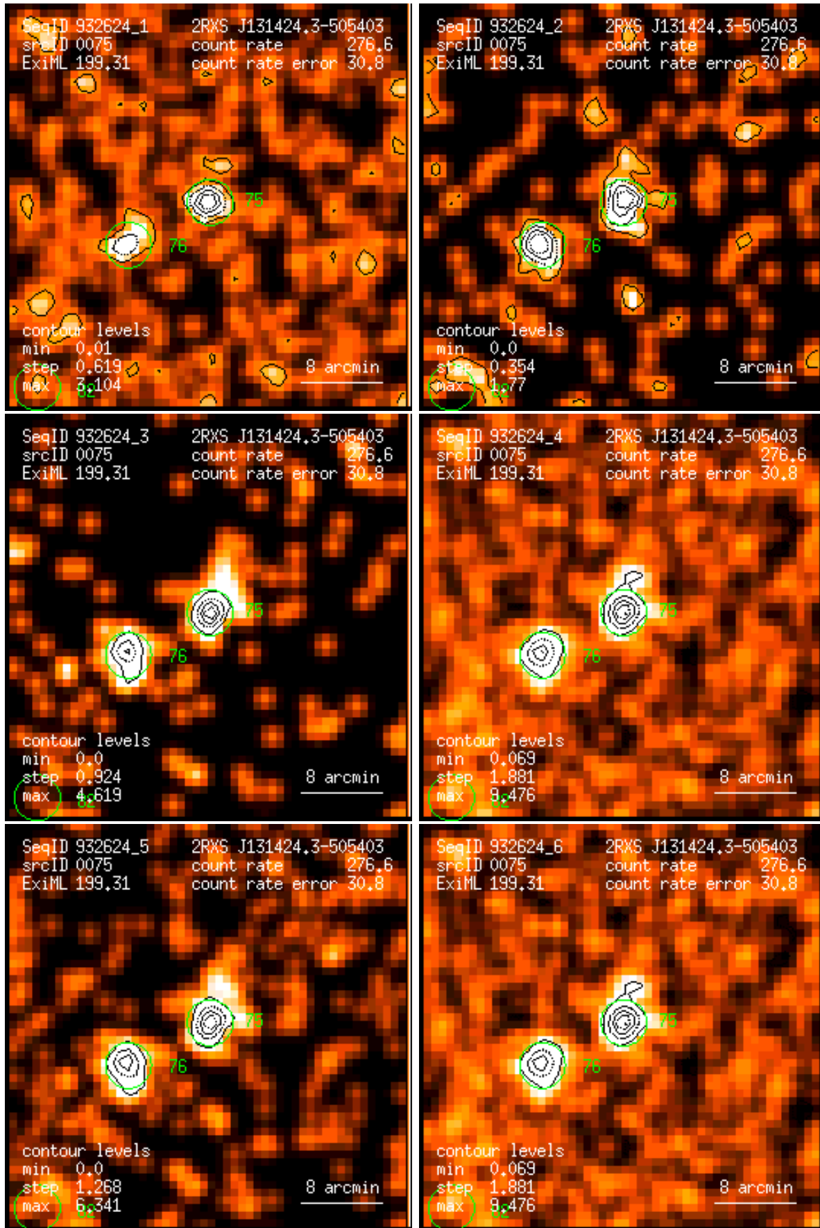
Figure 75: RASS 932624: detection 0075: band rate images, Gaussian filter: (1) PSPC channels 11 – 41, (2) 52 – 90, (3) 91 – 201, (4) 11 – 235, (5) 52 – 201, (6) 11 – 201. Broad band rates in counts/ks. Band rate contour levels in counts/ks/arcmin 2 .
