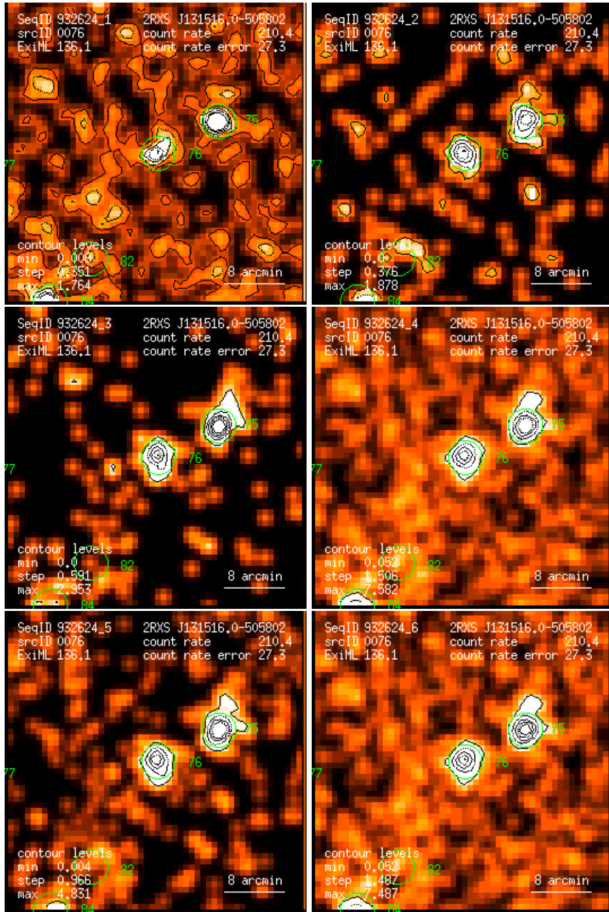
Figure 76: RASS 932624: detection 0076: band rate images, Gaussian filter: (1) PSPC channels 11 – 41, (2) 52 – 90, (3) 91 – 201, (4) 11 – 235, (5) 52 – 201, (6) 11 – 201. Broad band rates in counts/ks. Band rate contour levels in counts/ks/arcmin 2 .
