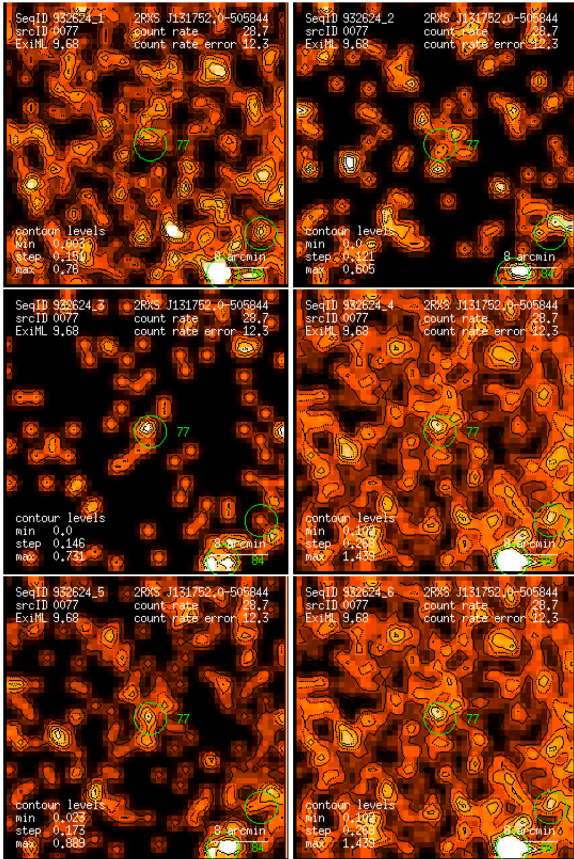
Figure 77: RASS 932624: detection 0077: band rate images, Gaussian filter: (1) PSPC channels 11 – 41, (2) 52 – 90, (3) 91 – 201, (4) 11 – 235, (5) 52 – 201, (6) 11 – 201. Broad band rates in counts/ks. Band rate contour levels in counts/ks/arcmin 2 .
