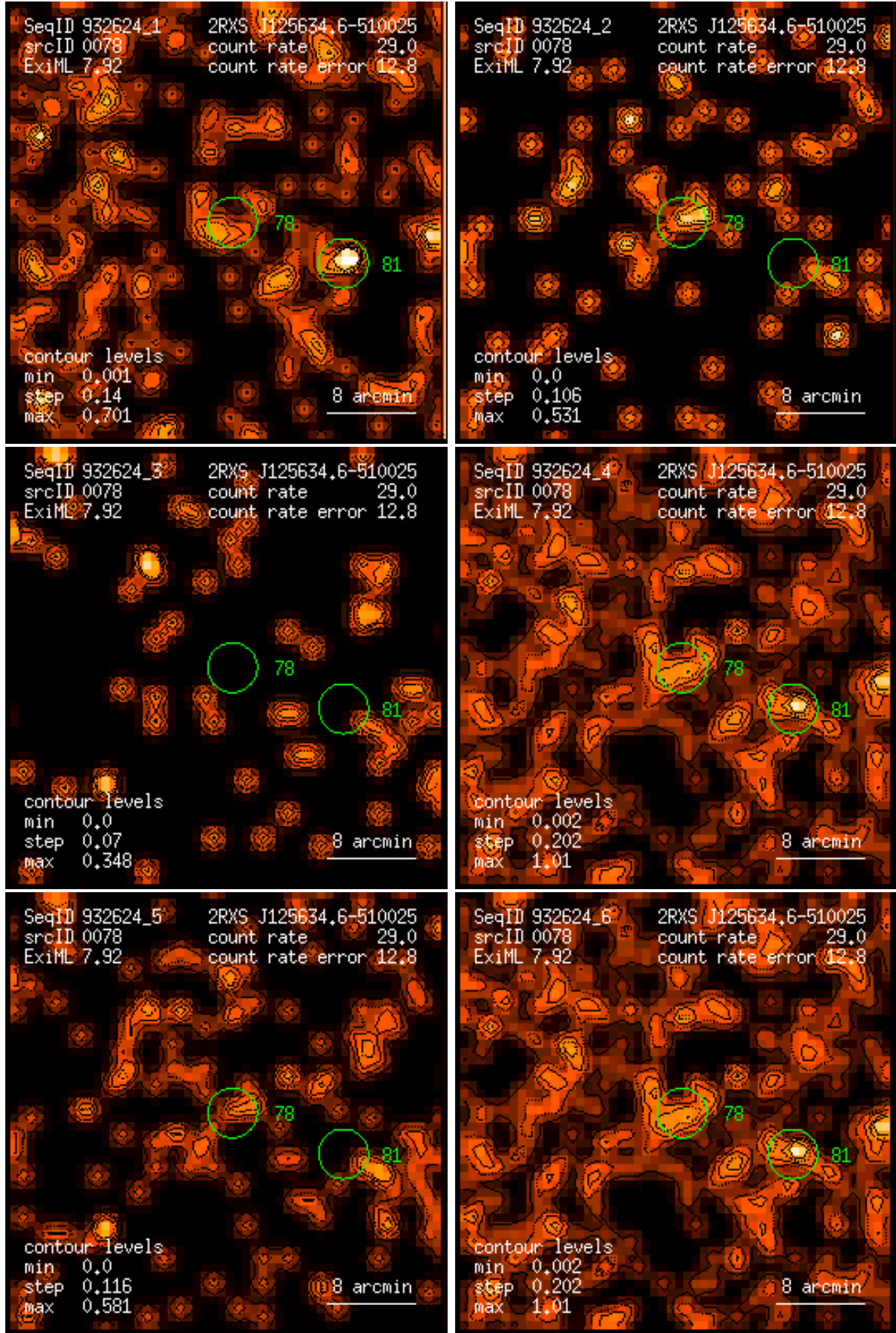
Figure 78: RASS 932624: detection 0078: band rate images, Gaussian filter: (1) PSPC channels 11 – 41, (2) 52 – 90, (3) 91 – 201, (4) 11 – 235, (5) 52 – 201, (6) 11 – 201. Broad band rates in counts/ks. Band rate contour levels in counts/ks/arcmin 2 .
