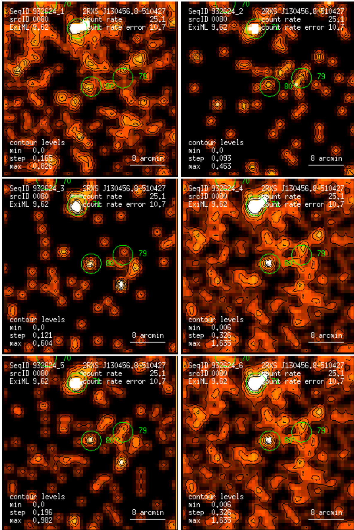
Figure 80: RASS 932624: detection 0080: band rate images, Gaussian filter: (1) PSPC channels 11 – 41, (2) 52 – 90, (3) 91 – 201, (4) 11 – 235, (5) 52 – 201, (6) 11 – 201. Broad band rates in counts/ks. Band rate contour levels in counts/ks/arcmin 2 .
