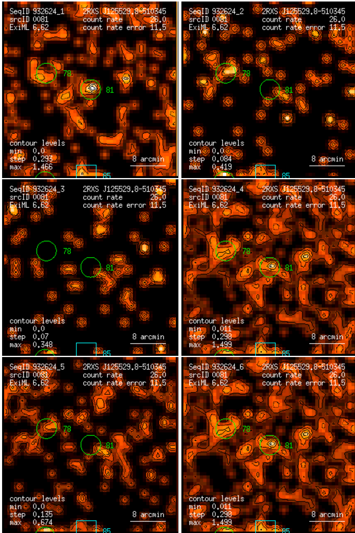
Figure 81: RASS 932624: detection 0081: band rate images, Gaussian filter: (1) PSPC channels 11 – 41, (2) 52 – 90, (3) 91 – 201, (4) 11 – 235, (5) 52 – 201, (6) 11 – 201. Broad band rates in counts/ks. Band rate contour levels in counts/ks/arcmin 2 .
