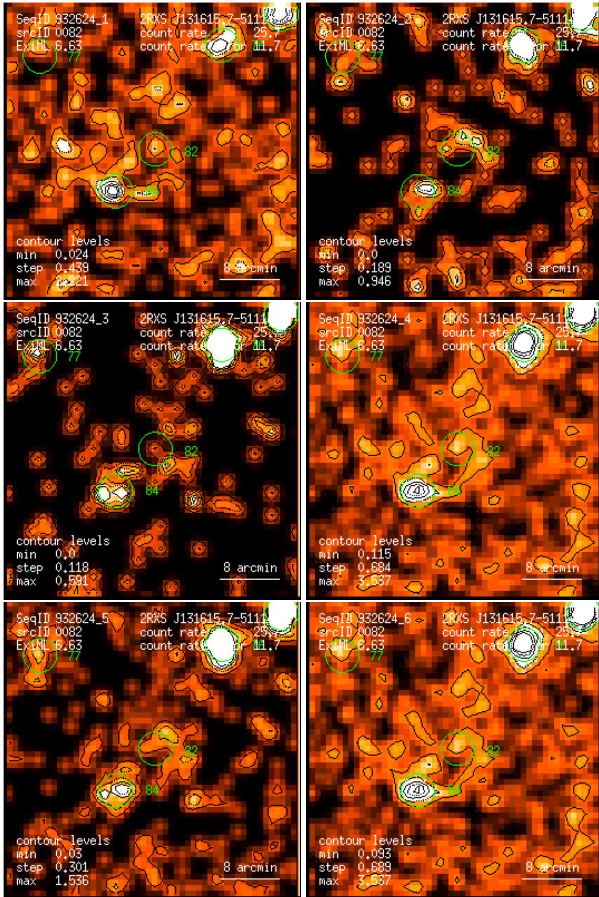
Figure 82: RASS 932624: detection 0082: band rate images, Gaussian filter: (1) PSPC channels 11 – 41, (2) 52 – 90, (3) 91 – 201, (4) 11 – 235, (5) 52 – 201, (6) 11 – 201. Broad band rates in counts/ks. Band rate contour levels in counts/ks/arcmin 2 .
