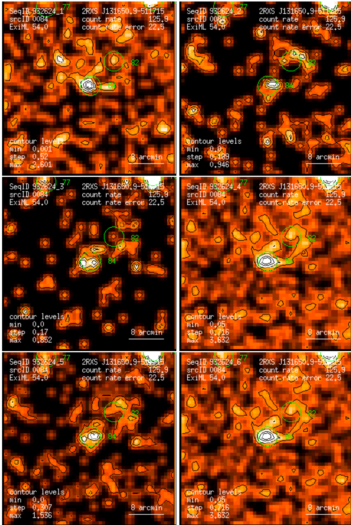
Figure 84: RASS 932624: detection 0084: band rate images, Gaussian filter: (1) PSPC channels 11 – 41, (2) 52 – 90, (3) 91 – 201, (4) 11 – 235, (5) 52 – 201, (6) 11 – 201. Broad band rates in counts/ks. Band rate contour levels in counts/ks/arcmin 2 .
