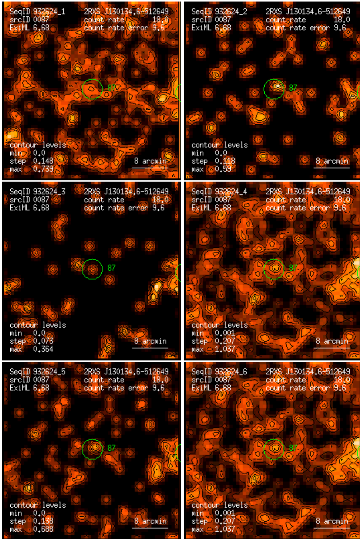
Figure 87: RASS 932624: detection 0087: band rate images, Gaussian filter: (1) PSPC channels 11 – 41, (2) 52 – 90, (3) 91 – 201, (4) 11 – 235, (5) 52 – 201, (6) 11 – 201. Broad band rates in counts/ks. Band rate contour levels in counts/ks/arcmin 2 .
