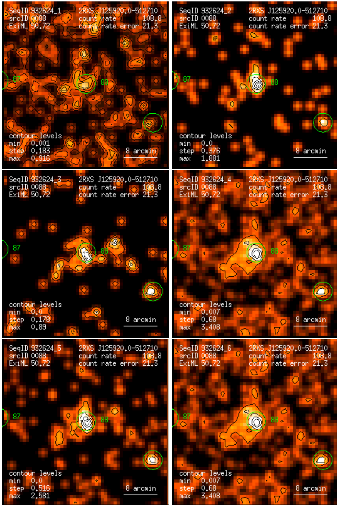
Figure 88: RASS 932624: detection 0088: band rate images, Gaussian filter: (1) PSPC channels 11 – 41, (2) 52 – 90, (3) 91 – 201, (4) 11 – 235, (5) 52 – 201, (6) 11 – 201. Broad band rates in counts/ks. Band rate contour levels in counts/ks/arcmin 2 .
