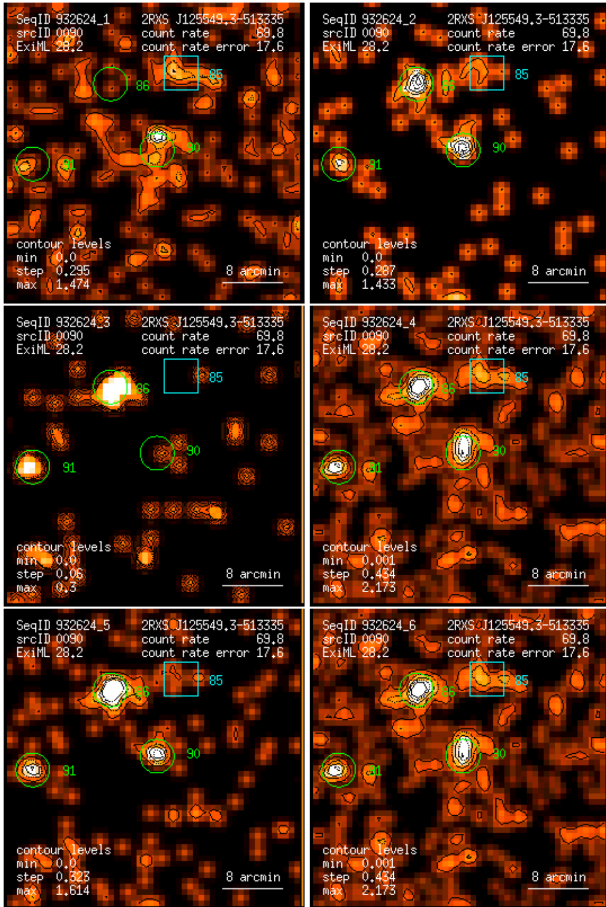
Figure 90: RASS 932624: detection 0090: band rate images, Gaussian filter: (1) PSPC channels 11 – 41, (2) 52 – 90, (3) 91 – 201, (4) 11 – 235, (5) 52 – 201, (6) 11 – 201. Broad band rates in counts/ks. Band rate contour levels in counts/ks/arcmin 2 .
