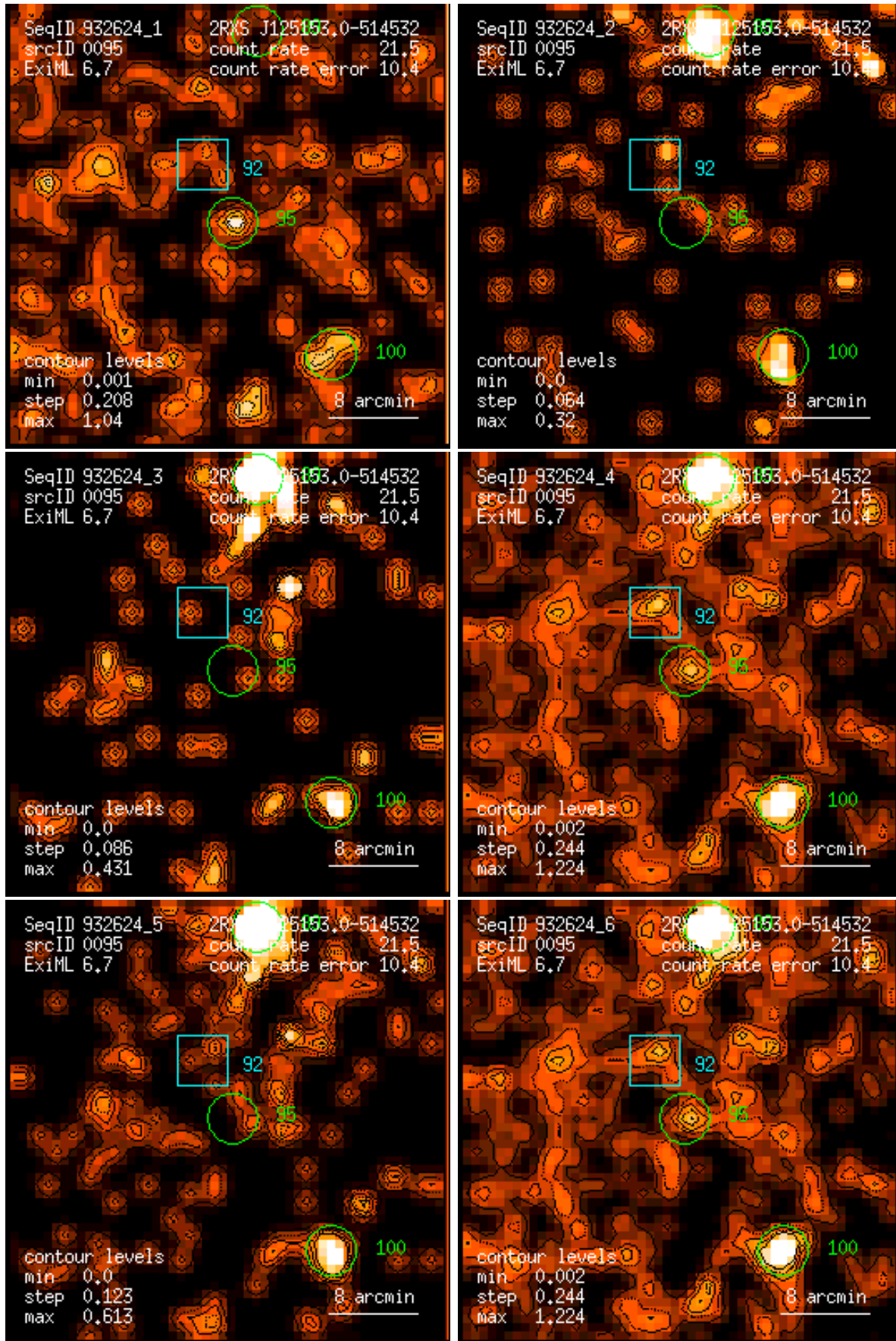
Figure 95: RASS 932624: detection 0095: band rate images, Gaussian filter: (1) PSPC channels 11 – 41, (2) 52 – 90, (3) 91 – 201, (4) 11 – 235, (5) 52 – 201, (6) 11 – 201. Broad band rates in counts/ks. Band rate contour levels in counts/ks/arcmin 2 .
