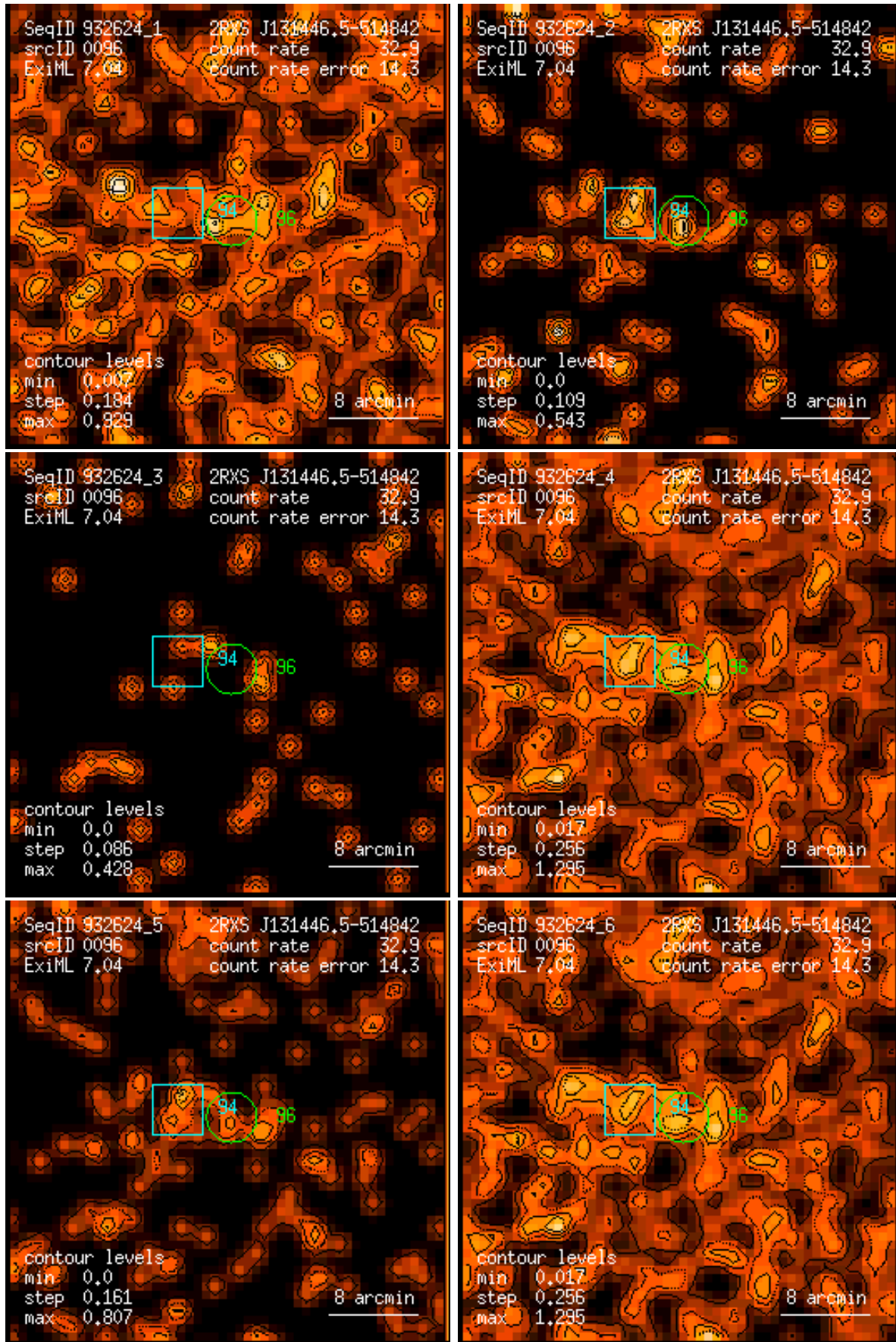
Figure 96: RASS 932624: detection 0096: band rate images, Gaussian filter: (1) PSPC channels 11 – 41, (2) 52 – 90, (3) 91 – 201, (4) 11 – 235, (5) 52 – 201, (6) 11 – 201. Broad band rates in counts/ks. Band rate contour levels in counts/ks/arcmin 2 .
