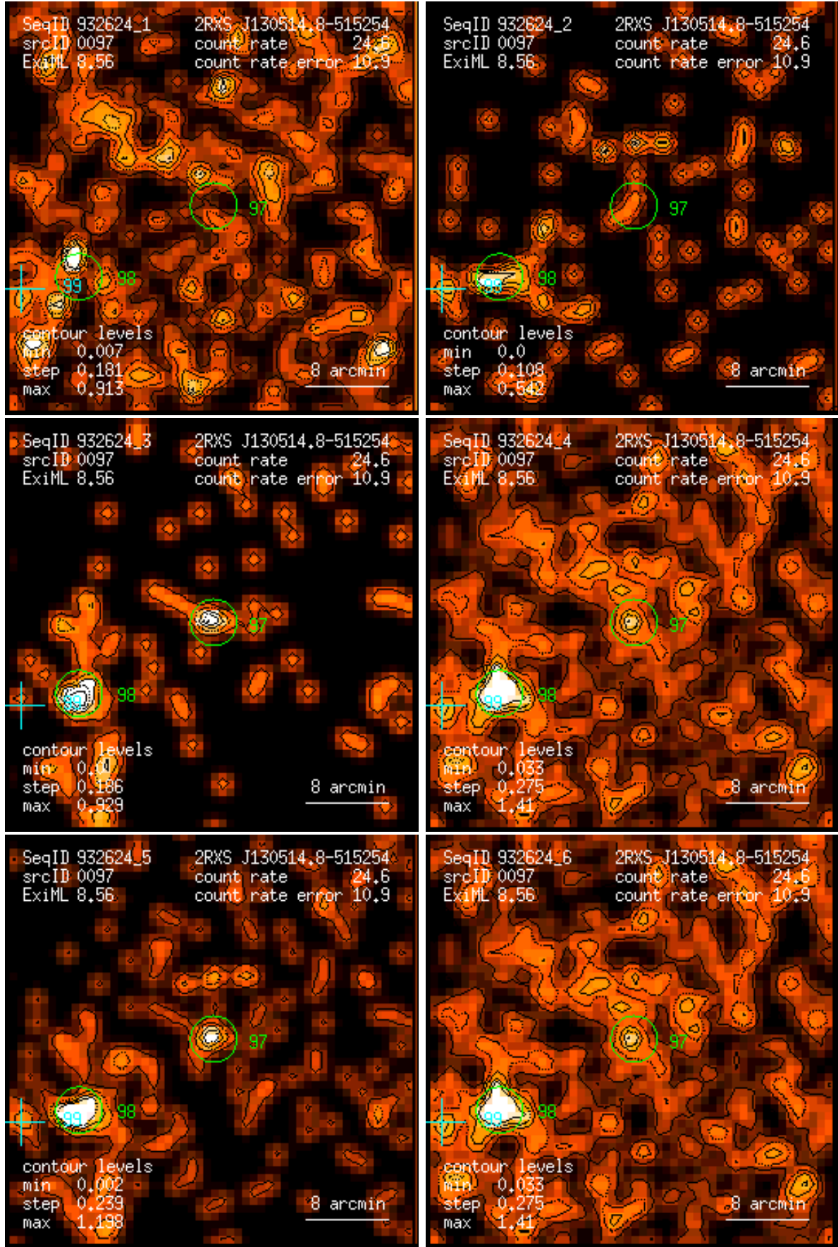
Figure 97: RASS 932624: detection 0097: band rate images, Gaussian filter: (1) PSPC channels 11 – 41, (2) 52 – 90, (3) 91 – 201, (4) 11 – 235, (5) 52 – 201, (6) 11 – 201. Broad band rates in counts/ks. Band rate contour levels in counts/ks/arcmin 2 .
