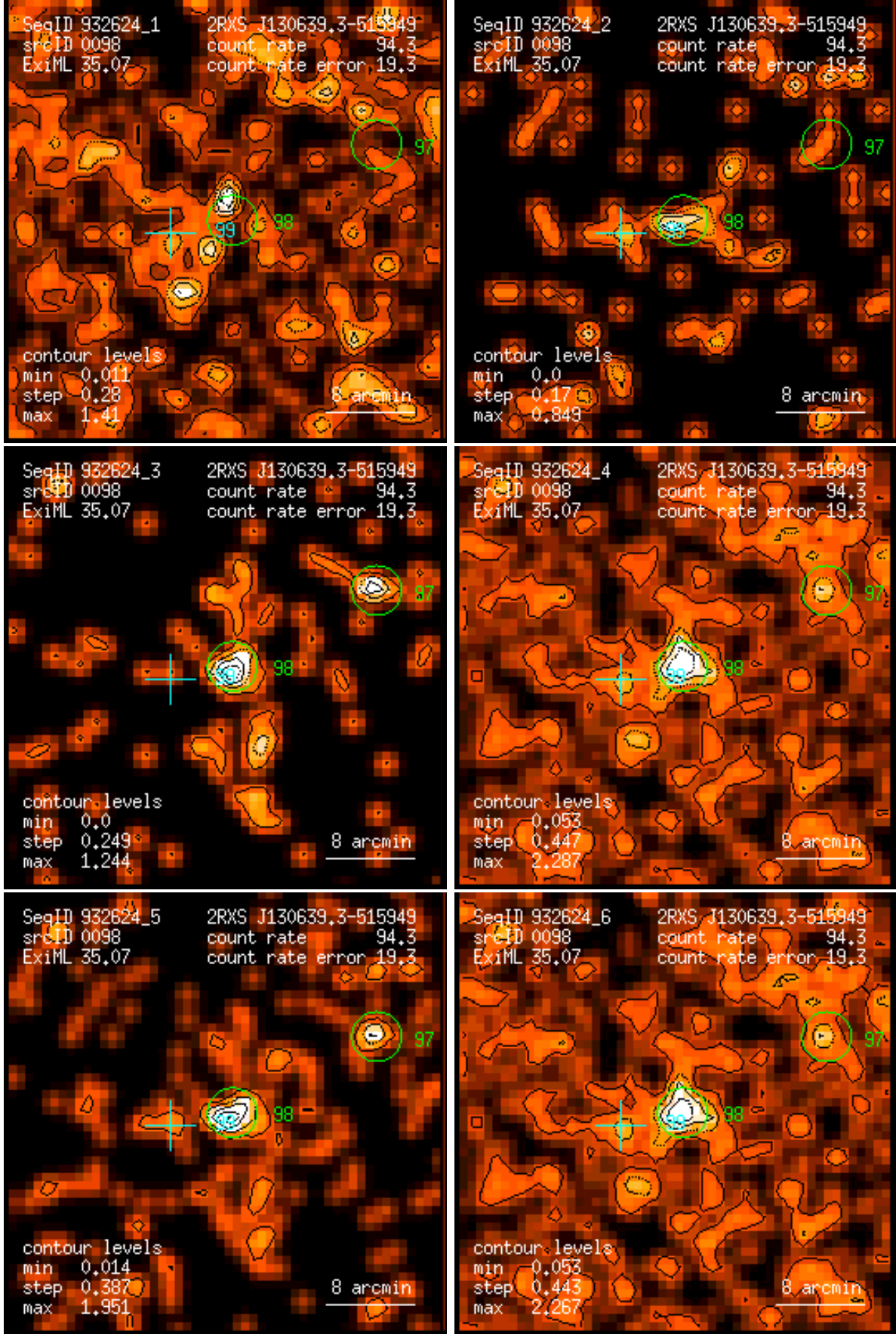
Figure 98: RASS 932624: detection 0098: band rate images, Gaussian filter: (1) PSPC channels 11 – 41, (2) 52 – 90, (3) 91 – 201, (4) 11 – 235, (5) 52 – 201, (6) 11 – 201. Broad band rates in counts/ks. Band rate contour levels in counts/ks/arcmin 2 .
